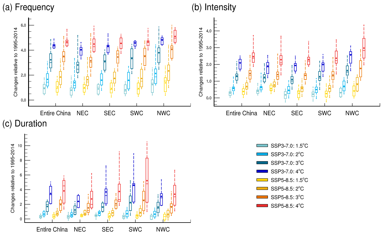
Fig. 5 Box plots of the regionally averaged changes in the frequency ( a , units: events a^{-1} ), intensity ( b , units: ^{\circ}C ) and duration ( c , units: days) of Compound HWs at 1.5 ^{\circ}C (2 ^{\circ}C , 3 ^{\circ}C , 4 ^{\circ}C ) GWL relative to the recent climate (1995–2014) under the two scenarios over the entire China and subregions. With each box, the horizontal lines
