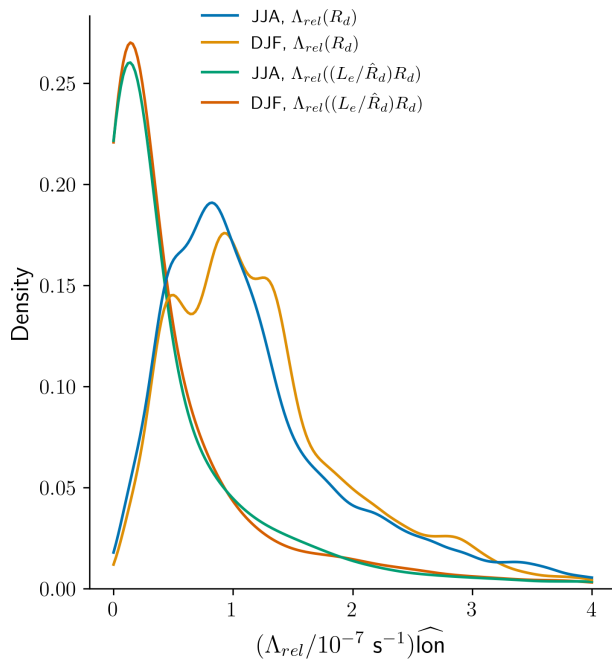
Figure 9. Kernel density estimation of (\Lambda_{\text{rel}}/10^{-7} \text{ s}^{-1})\widehat{\text{lon}} , where \widehat{\text{lon}} is a normalised longitude. The four curves represent the dissipation rate \Lambda_{\text{rel}} depending on the chosen eddy length scale and season (DJF or JJA). Values over the equator band between 5^\circ \text{ S} and 5^\circ \text{ N} are not included here.
