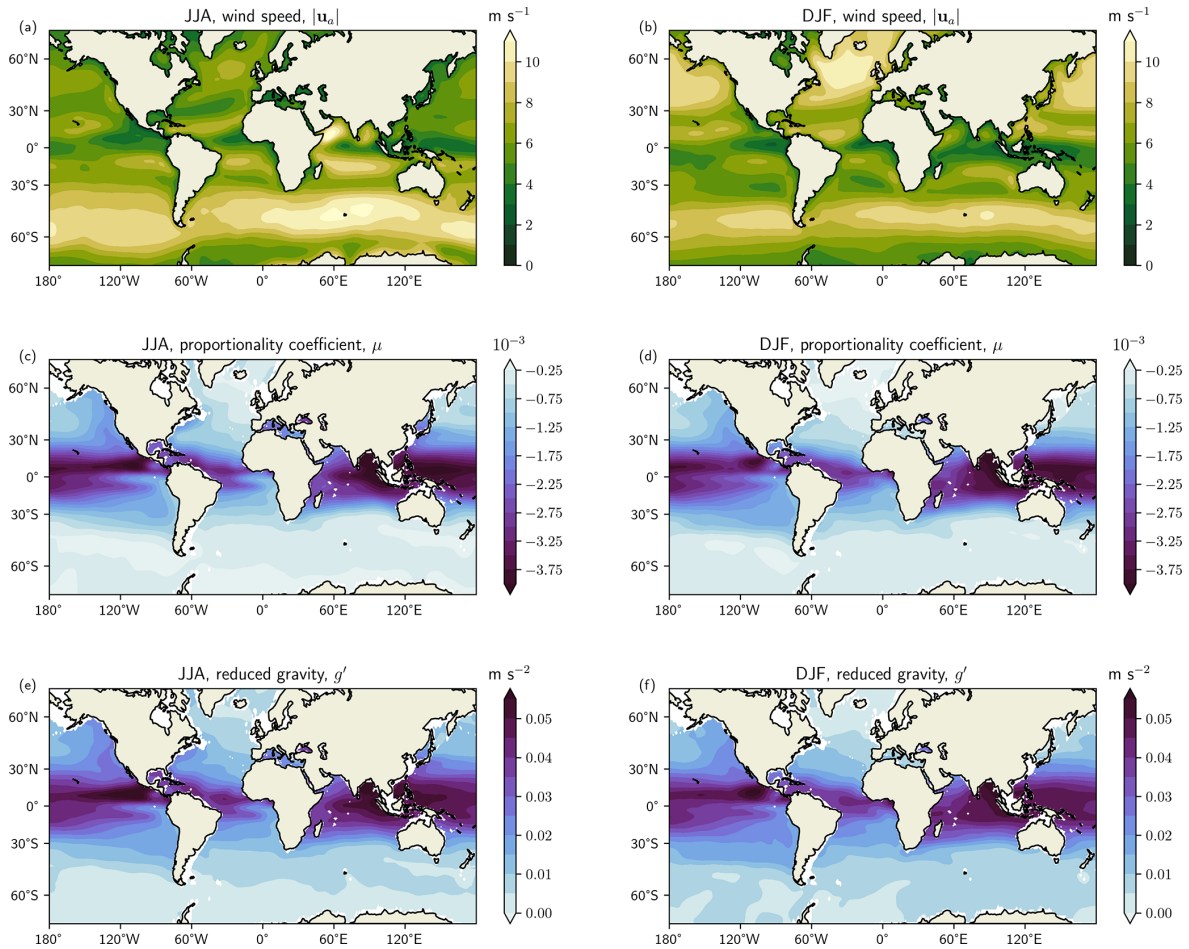
Figure 6. Global maps between the latitudes of 70° S and 70° N displaying contributions to the dissipation rate, \Lambda_{rel} , for (a, c, e) June–July–August (JJA) and (b, d, f) December–January–February (DJF). Panels (a, b) show wind speed, |u_a| (in m s^{-1} ), (c, d) proportionality coefficient, \mu , and (e, f) reduced gravity, g' (in m s^{-2} ). The data are calculated from World Ocean Atlas and NOAA datasets over the period 1981–2010.
