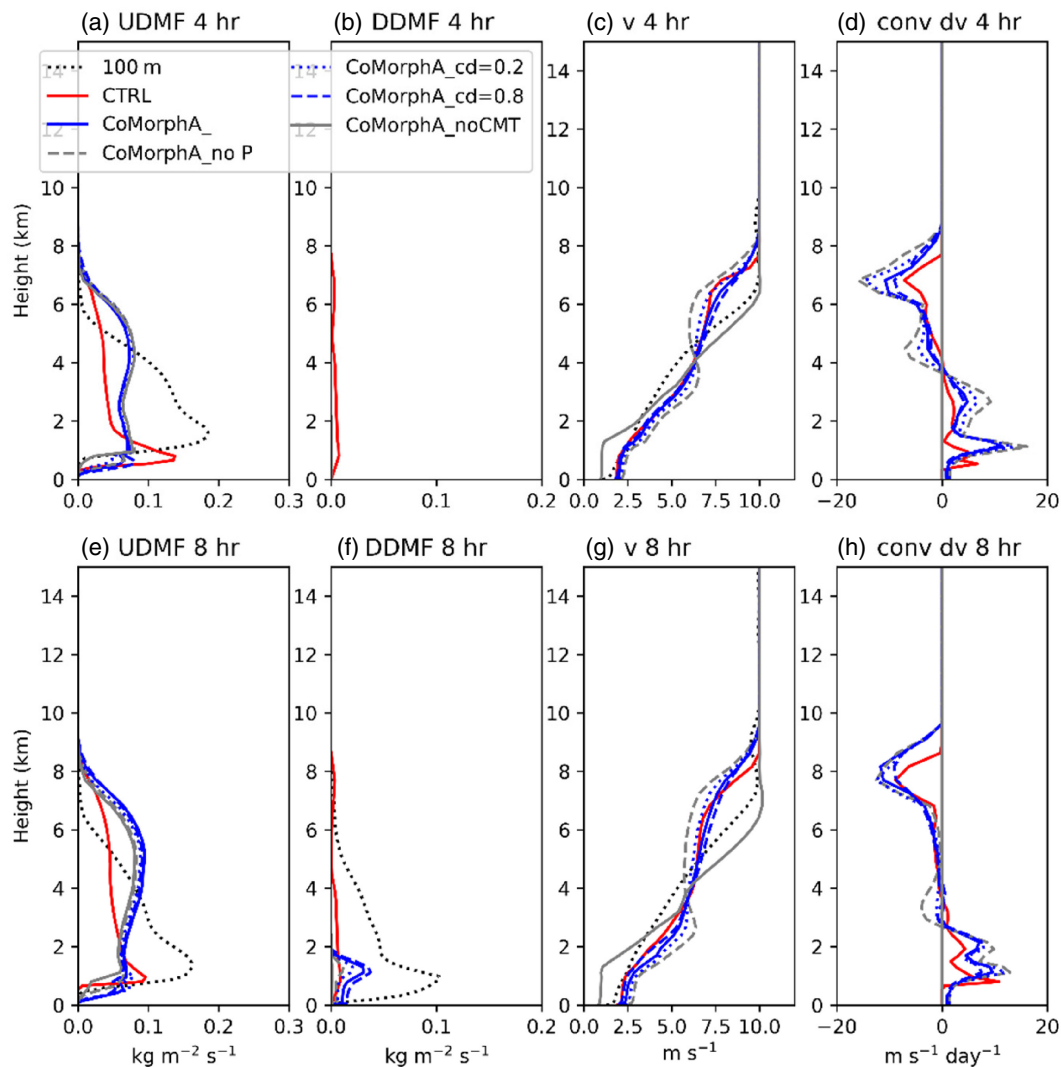
FIGURE 10 Convective momentum transport (CMT). Profiles at 4 hr of (a) updraught mass flux [ \text{kg}\cdot\text{m}^{-2}\cdot\text{s}^{-1} ], (b) downdraught mass flux [ \text{kg}\cdot\text{m}^{-2}\cdot\text{s}^{-1} ], (c) meridional wind [ \text{m}\cdot\text{s}^{-1} ] and (d) the increment in meridional wind due to convection [ \text{m}\cdot\text{s}^{-1}\cdot\text{day}^{-1} ] in the parametrized runs for the cold air outbreak case. (e–h) As (a–d) but 8 hr into the run. Results shown for the 100 m CRM (black), CTRL (red) and various configurations of CoMorph: CoMorph-A (blue, solid), CoMorph-A with no CMT (grey), CoMorph-A but no pressure term in the CMT calculation (grey, dashed), drag coefficient of 0.2 (blue, dotted) and 0.8 (blue, dashed).
