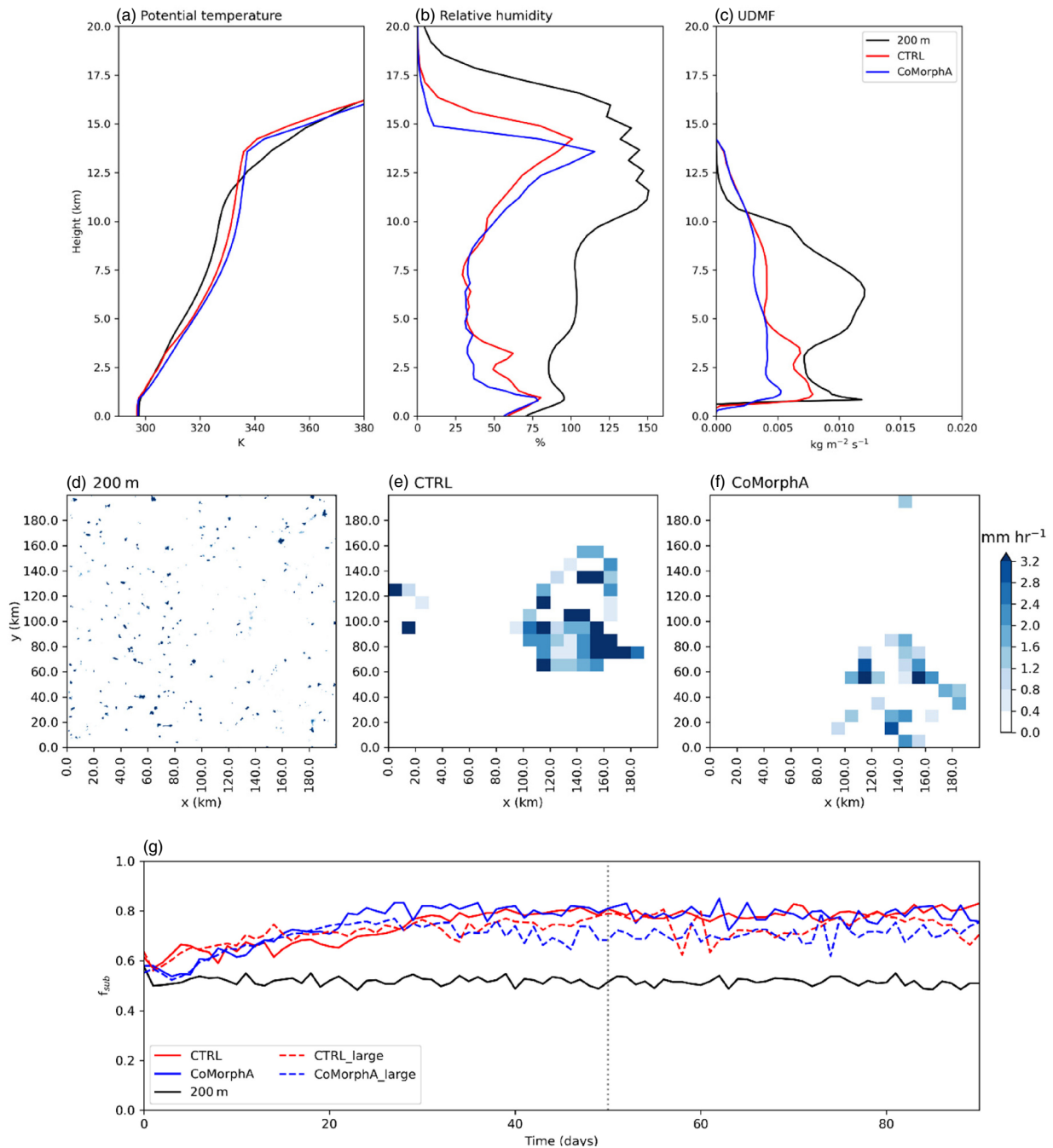
FIGURE 1 Radiative–convective equilibrium (RCE). Profiles of (a) potential temperature [K], (b) relative humidity [%], with respect to water (ice) above (below) 0^{\circ}\text{C} , and (c) updraught mass flux, averaged over the final 70 days of simulation. Snapshot of surface precipitation rate [ \text{mm}\cdot\text{hr}^{-1} ] on day 50 of the simulations from (d) 200 m CRM (native resolution), (e) CTRL and (f) CoMorph-A, both 10 km resolution, (g) time series of f_{\text{sub}} , calculated as in the text, for the CRM, CTRL and CoMorph-A. The dashed lines are the CTRL and CoMorph-A results over the large 6000 \times 400 \text{ km}^2 domain. The vertical grey dotted line in (g) shows the timing of the snapshots in (d–f).
