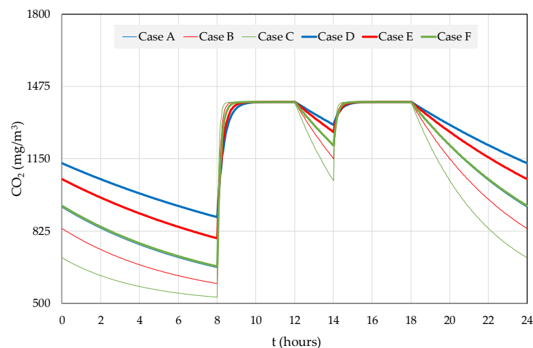
Figure 21. Evolution of CO 2 concentration for the six cases studied.
