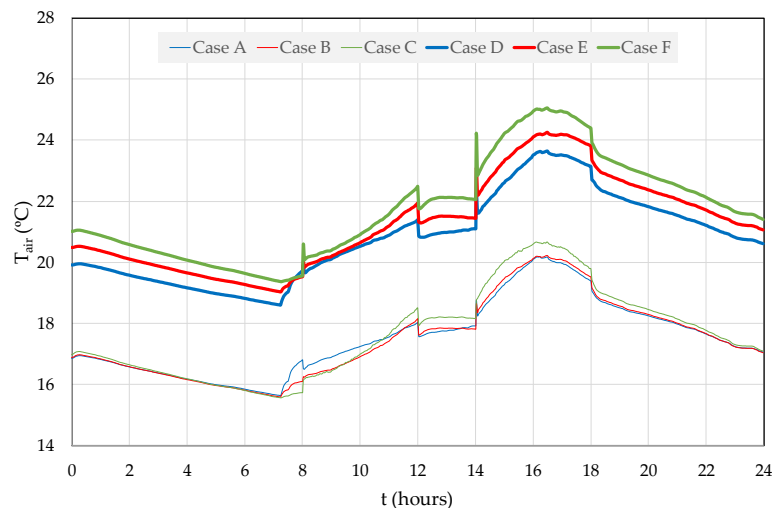
Figure 22. Evolution of internal air temperature ( T_{\text{air}} ) for the six cases studied.
