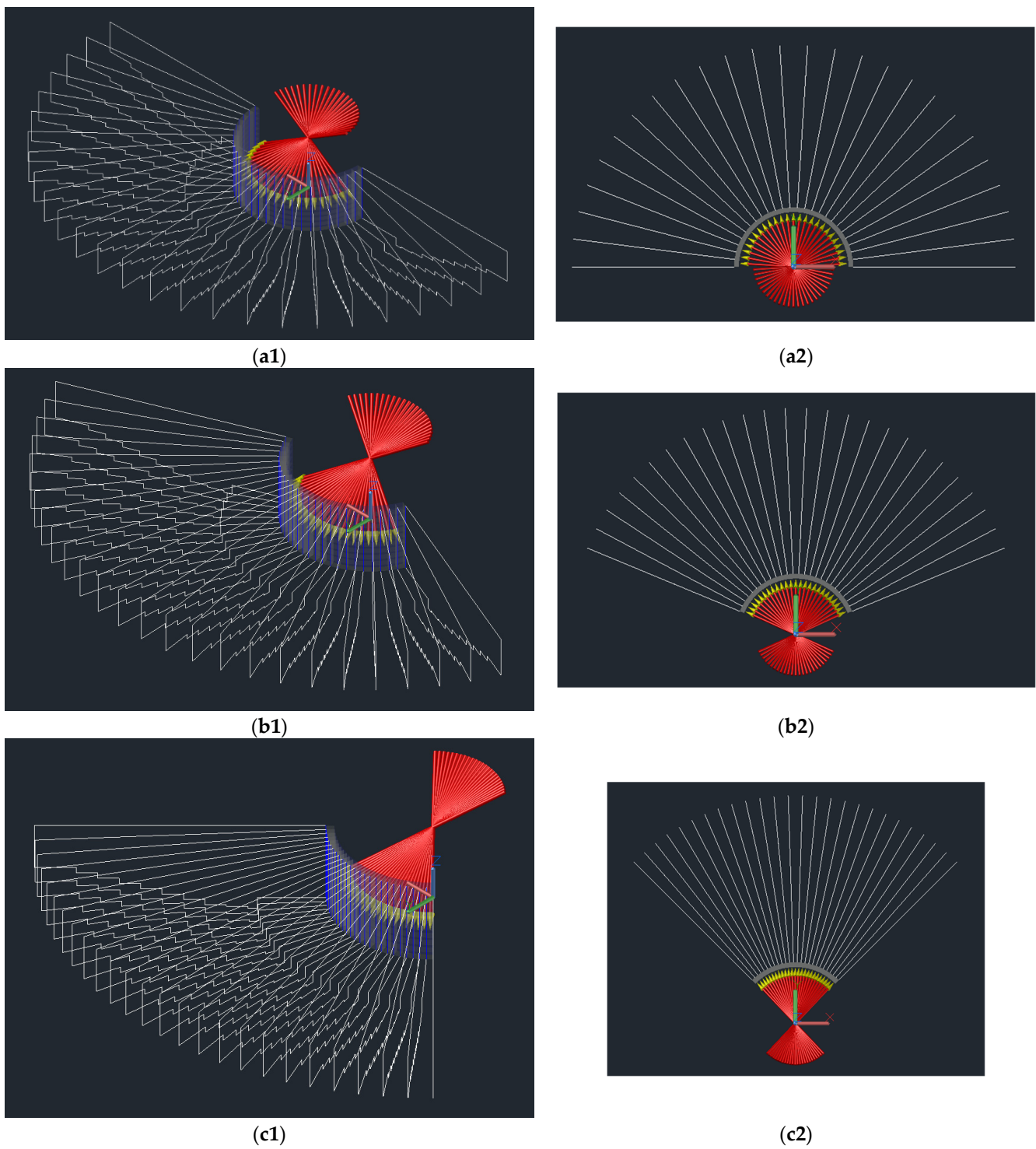
Figure 5. Scheme of the auditorium construction methodology, using a two-dimensional vertical section, and the semi-circular DSF solar radiation. (a1,a2) Case A, (b1,b2) Case B, and (c1,c2) Case C. Figures with index 1 represent the three-dimensional southeast view of the semi-circular DSF and the auditorium, while Figures with index 2 represent the top view.
