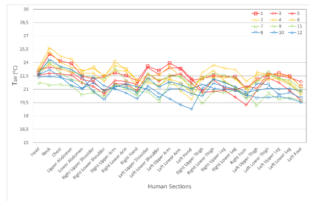
Figure 6. Air temperature ( T_{air} ) distribution around the occupants for a) Case A, b) Case B, and c) Case C).
