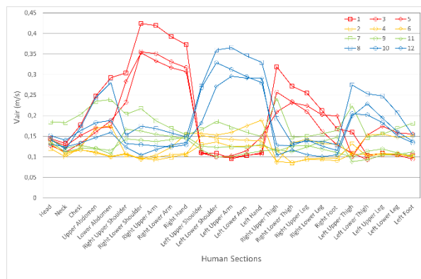
Figure 5. Air velocity ( V_{air} ) distribution around the occupants for a) Case A, b) Case B, and c) Case C).
