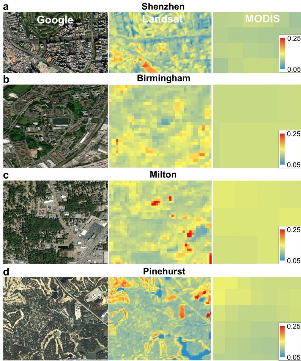
Fig. S7. Comparisons between Landsat and MODIS in capturing heterogeneous albedo of urban area over (a) Shenzhen, China, (b) Birmingham, , United Kingdom, (c) Milton, Florida, United States, and (d) Pinehurst, North Carolina, United States. First column: Google Basemap image. Middle column: Landsat-derived albedo. Third column: MODIS albedo.
