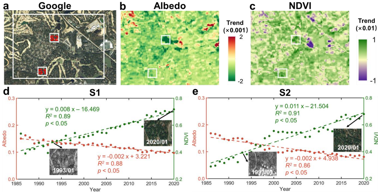
Fig. 13. Examples of close association between surface albedo and urban greening in the Pinehurst city, North Carolina, based on the maps of (a) Google Earth satellite image, (b) albedo trend, (c) NDVI trend, (d) time series of urban NDVI and albedo for the S1 area in (a), and (e) time series of urban NDVI and albedo for the S2 area in (a).
