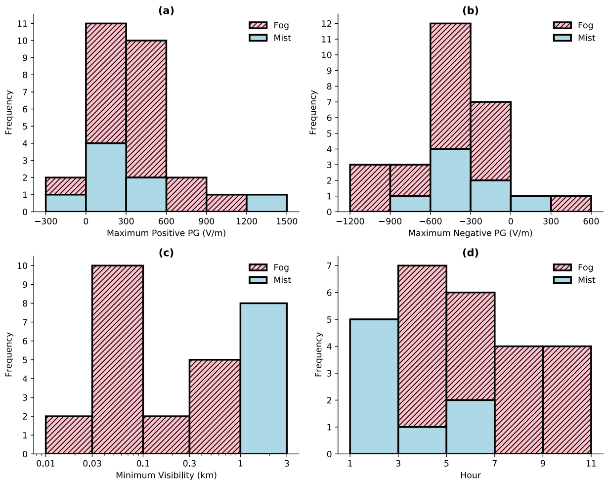
Figure 5. Stacked histograms of (a) maximum positive PG, (b) maximum negative PG, (c) minimum visibility, and (d) fog duration, during 19 dense fog events and 8 light fog events at Sanad Academy in 2021. Fog events were defined as instances when visibility was \leq 1 km, while mist events were characterised by visibility > 1 km and \leq 3 km (with RH > 90\% in both conditions). Minimum visibility data are presented on a logarithmic scale.
