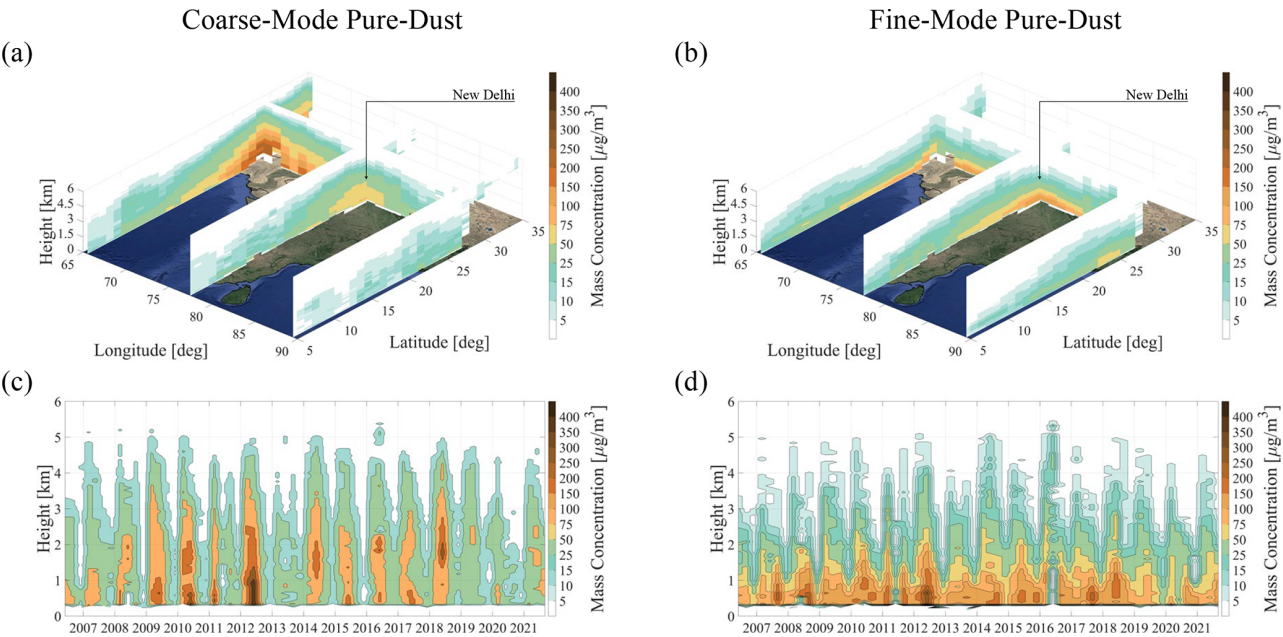
Figure 12. Coarse-mode (a) and fine-mode (b) pure-dust annual mean mass concentration cross-sections over the Indian Peninsula (lat: 28.5° N – long: 76.5° E – June 2006–December 2021) and seasonal mean mass concentration time series over the New Delhi megacity area (lat: 27–29° N – long: 76–78° E) for the coarse mode (c) and fine mode (d). Layer background: © Google Maps.
