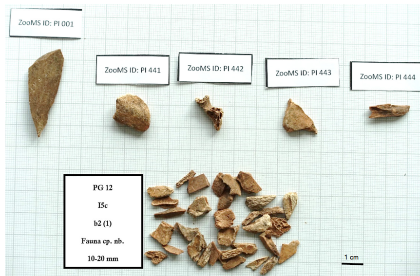
Figure 2. Examples of morphologically unidentifiable material from Le Piage recovered through water screening of the tapho-facies b sediments, Early Aurignacian layer (as defined by Bordes et al. 2011), sub-square I5c. Bones larger than 15mm were given a ZooMS ID and included in the ZooMS analysis, whereas bones smaller than 15mm were excluded (abbreviations: cp=compact ; nb=non burnt).
