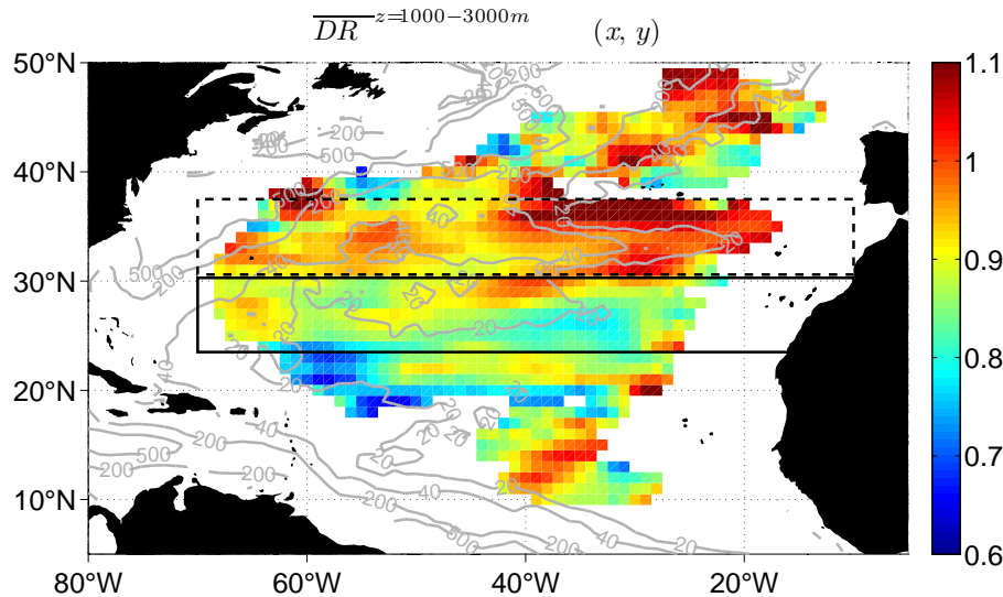
Fig. 11. Depth-to-surface speed Ratio averaged between 1000 and 3000 m ( \overline{DR}^{z=1000-3000\text{ m}}(x, y) , colours). Smoothed bottom topography is shown in black (contour interval 1000 m), EKE at 100 m is shown in grey (selected values indicated in \text{cm}^2 \text{s}^{-2} ). Rectangles indicates the regions over which DR(z) is averaged and discussed (left panel in Fig. 12, see Sect. 4.2).
