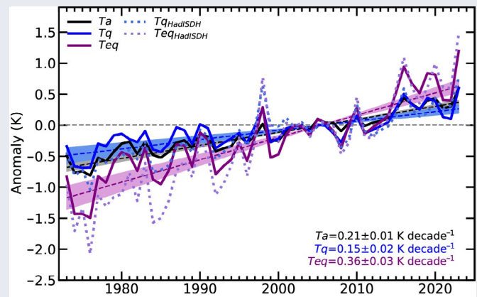
Fig. SB.2.3. 1973–2023 ERA5 and HadISDH trends in global mean air temperature ( T_a ; ERA5 only), latent temperature ( T_q = Teq - T_a ), and equivalent temperature ( Teq ). Trend lines were computed with simple linear regression, and shading spans 95% confidence intervals. The trends presented on the plot are for ERA5, with \pm 1 sigma standard error.
