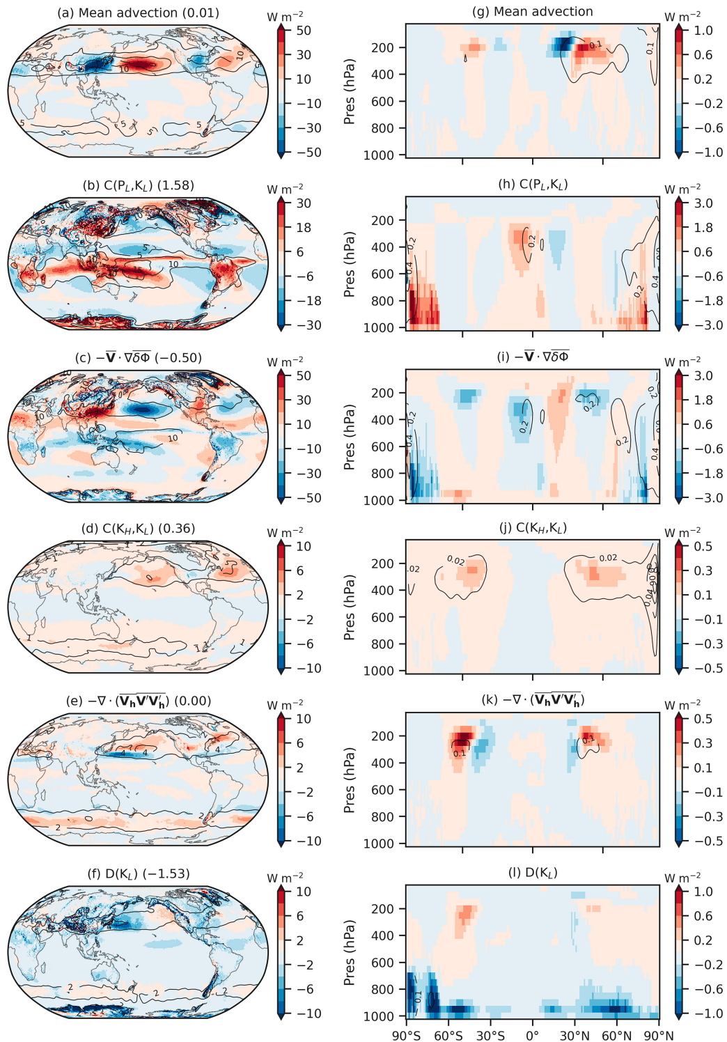
FIG. 5. The distribution of climatological budget terms for low-frequency KE ( W m^{-2} ). Vertically integrated (1000–50 hPa; mass-weighted) (a) mean advection, (b) conversion from low-frequency APE to KE C(P_L, K_L) , (c) mean advection of low-frequency geopotential anomaly with respect to reference state -\bar{\mathbf{V}} \cdot \nabla \delta \Phi , (d) conversion from high-frequency to low-frequency KEs C(K_H, K_L) , (e) convergence of the mean flux of meridional momentum in meridional direction -\nabla \cdot (\bar{\mathbf{V}}_h \bar{\mathbf{V}}_h') , and (f) dissipation of low-frequency KE D(K_L) in the boreal winter (December–February) during 1980–2021. (g)–(l) As in (a)–(e), but for zonal averages over the globe. The values in parentheses represent the global mean of conversion terms. The contours denote the annual standard deviation. The term \mathbf{V} represents three-dimensional wind including both horizontal and vertical components. The term \mathbf{V}_h denotes horizontal wind.
