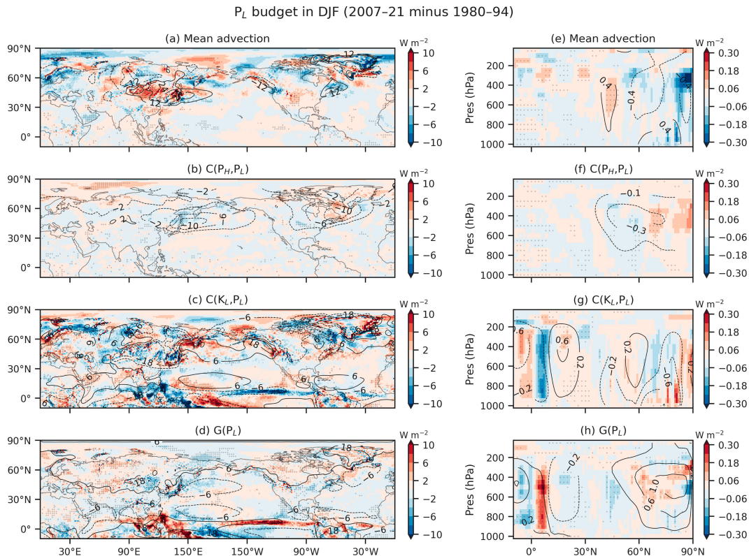
FIG. 8. The long-term changes in the budget of low-frequency APE budget ( \text{W m}^{-2} ) in the boreal winter (December–February) between 2007–21 and 1980–94. (a) Mean advection (shading), (b) conversion from high-frequency to low-frequency APEs C(P_H, P_L) , (c) conversion from low-frequency KE to APE C(K_L, P_L) , and (d) generation of low-frequency APE G(P_L) in the boreal winter (December–February) during 1980–2021. (e)–(h) As in (a)–(d), but for zonal averages over the globe. Black dots mark the grid points where the differences are at the 0.05 significance level according to the two-sided Student’s t test. The contours denote the long-term climatology during 1980–2021.
