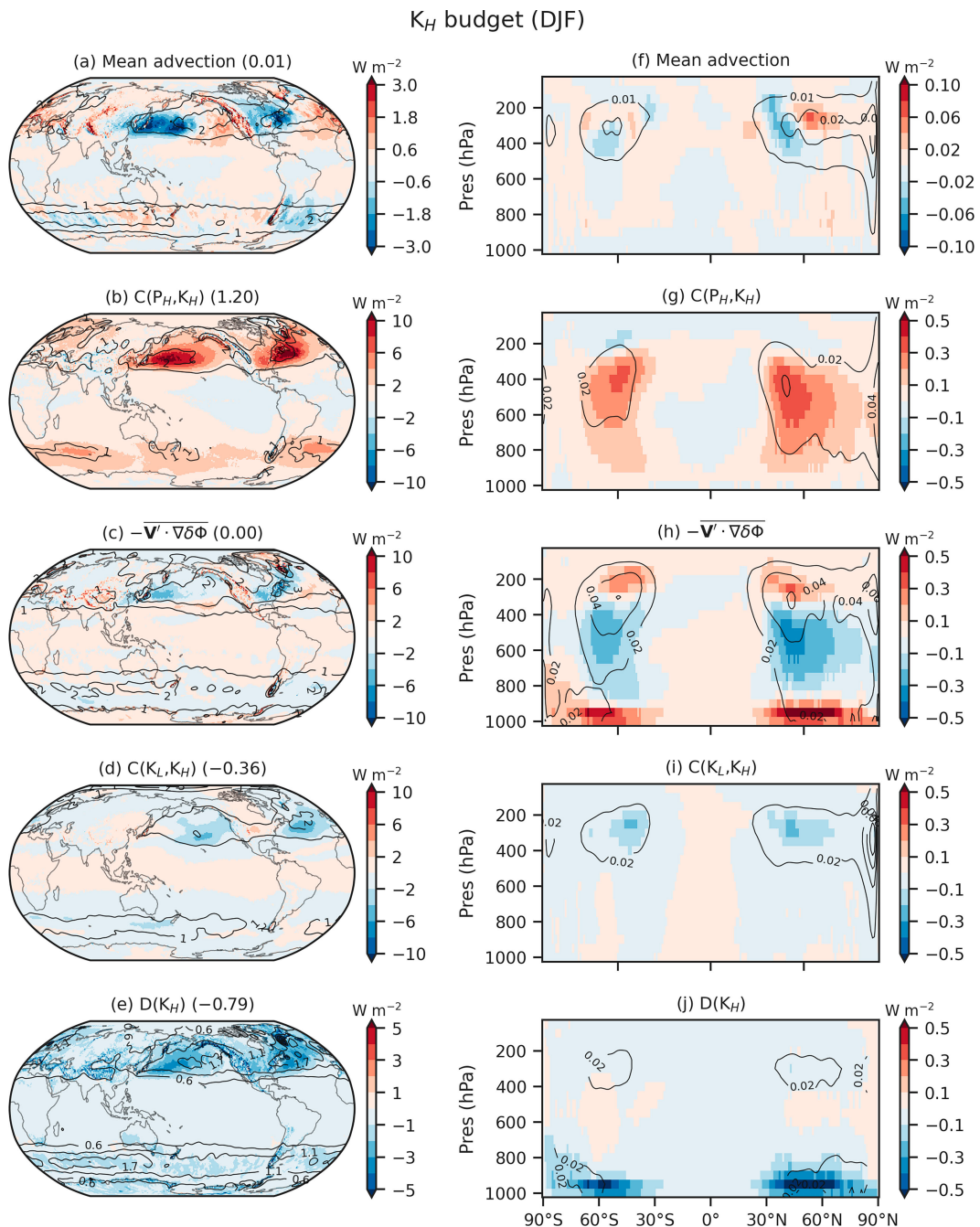
FIG. 4. The distribution of climatological budget terms for high-frequency KE ( W m^{-2} ). Vertically integrated (1000–50 hPa; mass-weighted) (a) mean advection (shading), (b) conversion from high-frequency APE to KE C(P_H, K_H) , (c) low-frequency eddy advection of high-frequency geopotential anomaly with respect to reference state -\overline{\mathbf{V}' \cdot \nabla \delta \Phi} , (d) conversion from low-frequency to high-frequency KEs C(K_L, K_H) , and (e) dissipation of high-frequency KE D(K_H) in the boreal winter (December–February) during 1980–2021. (f)–(j) As in (a)–(e), but for zonal averages over the globe. The values in parentheses represent the global mean of conversion terms. The contours denote the annual standard deviation. The term \mathbf{V} represents three-dimensional wind including both horizontal and vertical components.
