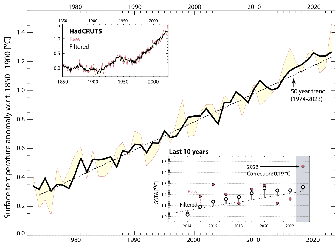
Fig. 3 | 50 years of global surface warming. All panels show global, annual mean surface temperature anomalies from the HadCRUT5 data series, raw (red) and SST influence filtered via a model-derived transfer function (black). The upper and lower
