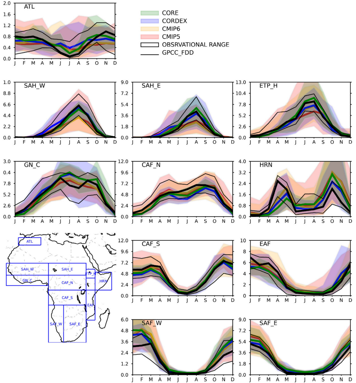
Fig. 3. Annual cycle of monthly averaged daily precipitation ( \text{mm d}^{-1} ) over the reference period (1981–2010) in the African subregions shown as blue boxes in the map. The thick black line represents the GPCC observed values, whereas the thin black lines show the range of a large ensemble of observational products, including reanalyses as well as satellite-based and gauge-based products. Colored lines and shaded areas show the ensemble mean and range of the different model ensembles, respectively. [Reprinted from Dosio et al. (2021b)].
