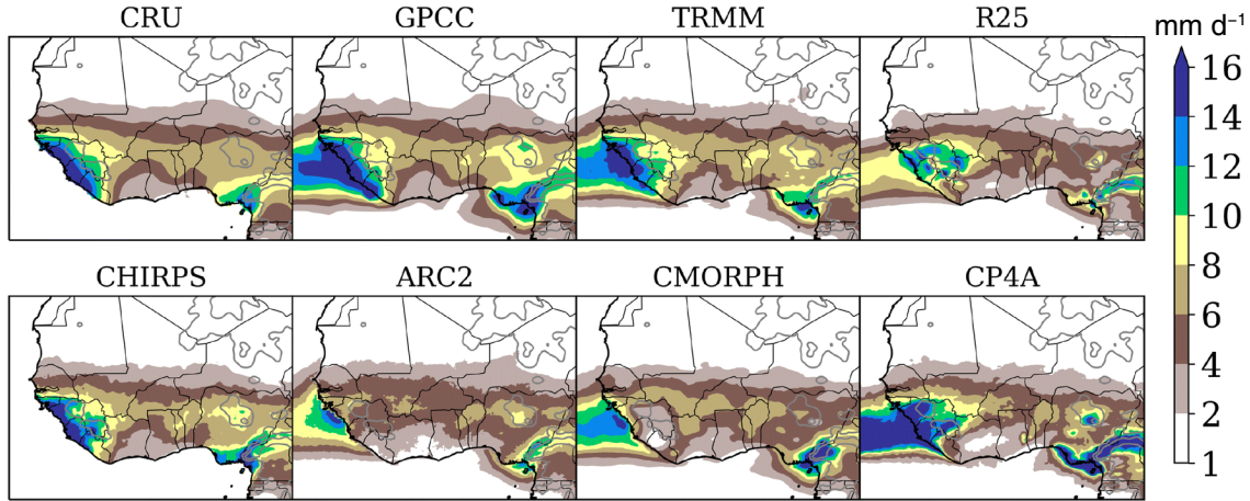
Fig. 4. Mean precipitation ( \text{mm d}^{-1} ) in JAS for different observed datasets, CRU, GPCC, TRMM, CHIRPS, ARC2, and CMORPH, and for a convection-permitting model (CP4A; at a 4.5 \times 4.5\text{-km} horizontal resolution at the equator) and a convection parameterized model (R25; at a 26 \times 39\text{-km} horizontal resolution at the equator). The average is computed over the period 1997–2006 (1998–2007) for CRU, GPCC, CHIRPS, ARC2, R25, and CP4A (TRMM and CMORPH). [Reprinted from Berthou et al. (2019)].
