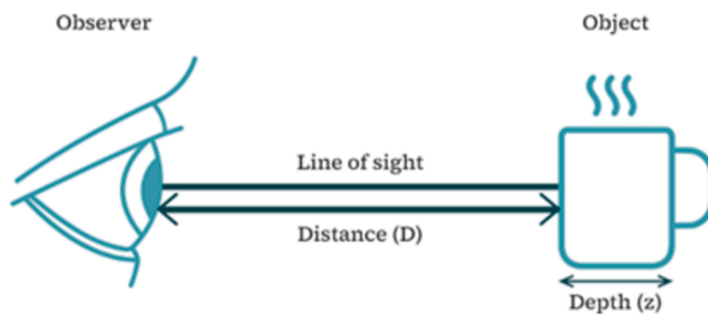
Fig. 3. Distance versus depth. Illustrating the difference between distance and depth in this work, showing the distance ( D ) from the observer to the object, and the depth ( z ) across the object.
