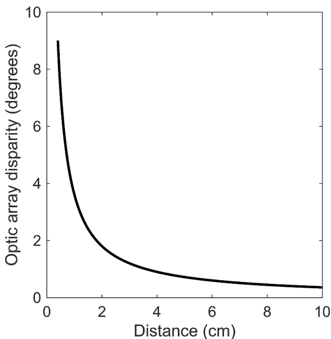
Fig. 2. Optic array disparity a as a function of distance, for a target directly in front of the observer, with an interocular distance of 63 mm.
