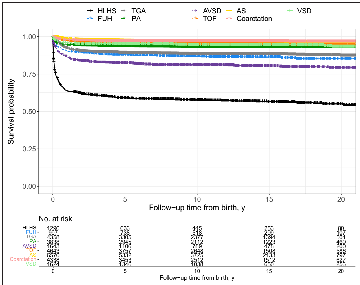
Figure 2. Kaplan–Meier survival curves for each congenital heart disease diagnosis. AS indicates aortic stenosis; AVSD, atrioventricular septal defect; FUH, functionally univentricular heart; HLHS, hypoplastic left heart syndrome; PA, pulmonary atresia; TGA, transposition of the great arteries; TOF, tetralogy of Fallot; and VSD, ventricular septal defect.
