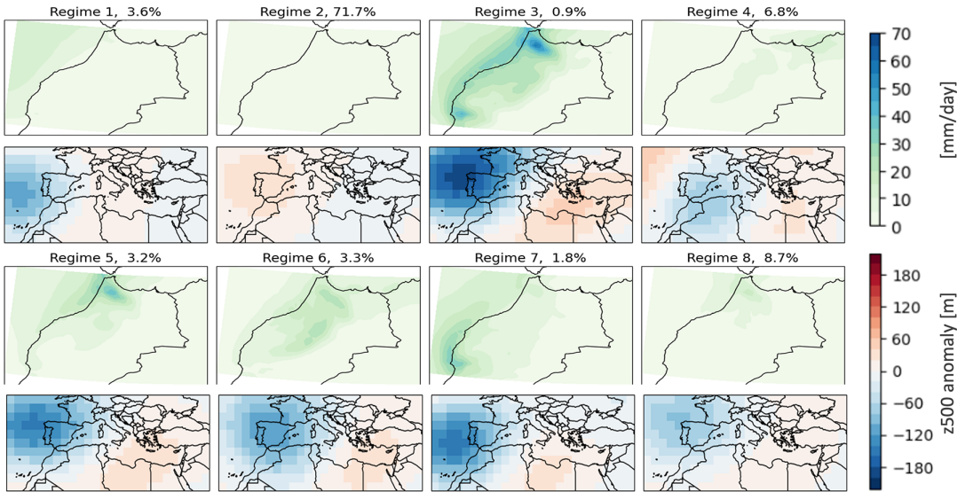
Figure 7. Precipitation clusters computed on precipitation reanalysis data without pre-processing using the k-means clustering algorithm for k=8 (top rows) and corresponding z500 anomalies (bottom rows).
