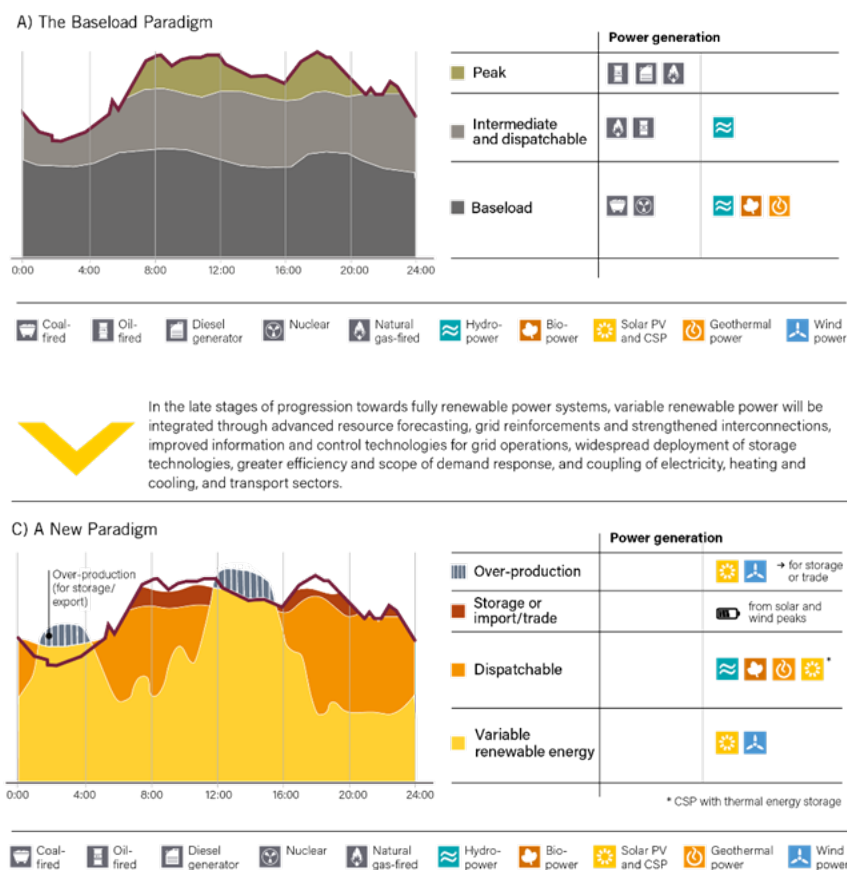
Figure 1.4. Illustration of the paradigm change in the power sector: (top) traditional baseload paradigm and (bottom) new, renewable generation based, paradigm
