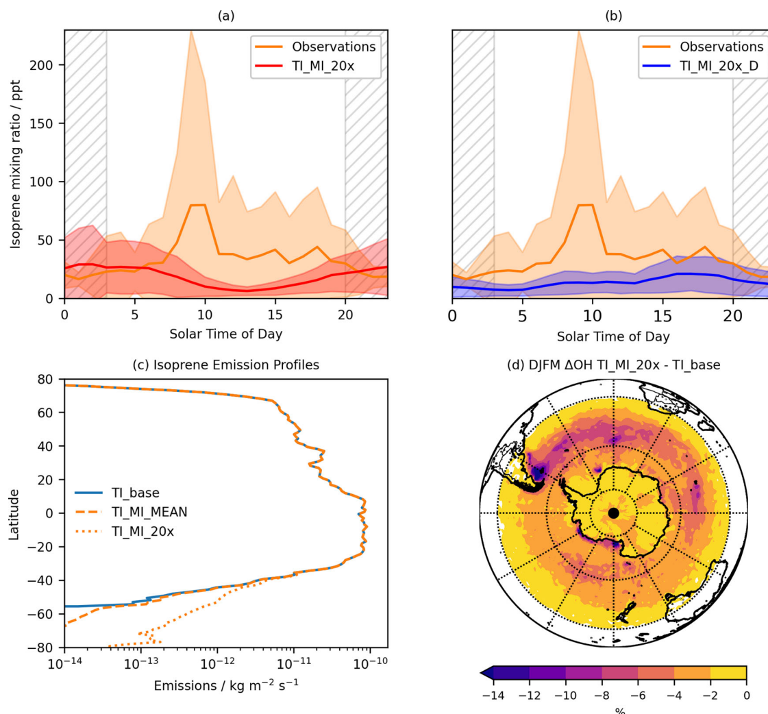
Fig. 4 | Isoprene diel cycle analysis and atmospheric impacts of enhanced isoprene emissions. Mean diel cycle of marine-only isoprene (orange line) along with the modelled diel cycles for (a) TI_{MI\_20x} and (b) TI_{MI\_20x\_D} for the entire Antarctic Circumnavigation Expedition (ACE). The gray-hatched areas indicate nighttime (the length of which varies by \pm 1 h throughout the cruise); shaded areas represent 1 standard deviation above and below each 1-h mean. See Fig. S15 for the diel cycles of the different legs of ACE. The 0 solar time of day corresponds to 00:00 local time and 23 corresponds to 23:00 local time. c Latitudinal profile of
