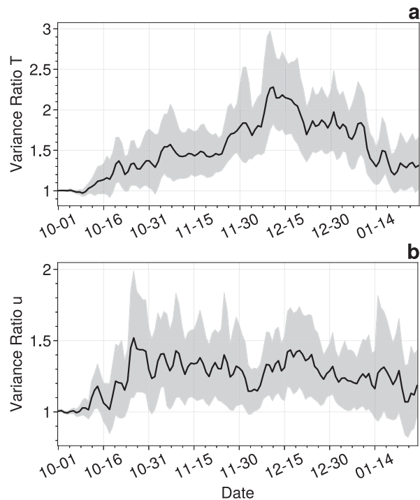
FIG. 6. Ratio of the variances in (a) 80-hPa polar cap temperature and (b) 60^{\circ} S zonal-mean zonal wind between RADINT and CTRL.
