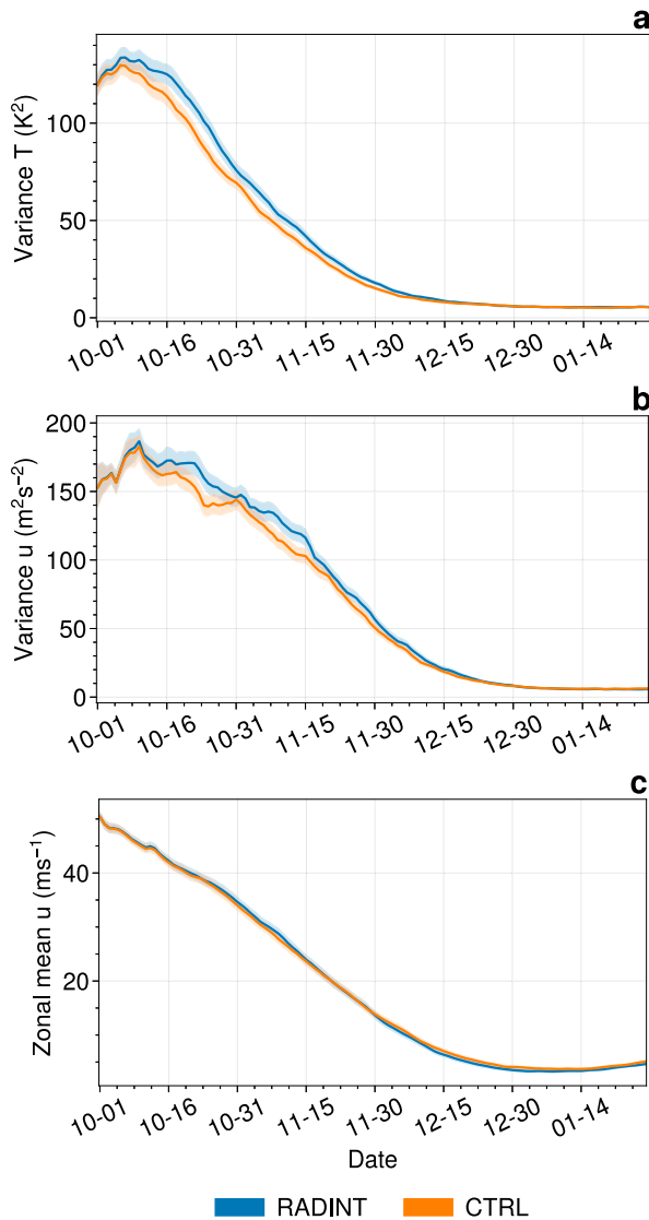
FIG. 10. (a),(b) The temperature ( K^2 ) and zonal wind ( m^2 s^{-2} ) variance about the zonal mean and (c) the zonal-mean zonal wind ( m s^{-1} ) for RADINT (blue) and CTRL (orange). The temperature variance is calculated at 60^\circ S and 80 hPa and the wind at 60^\circ S and 50 hPa.
