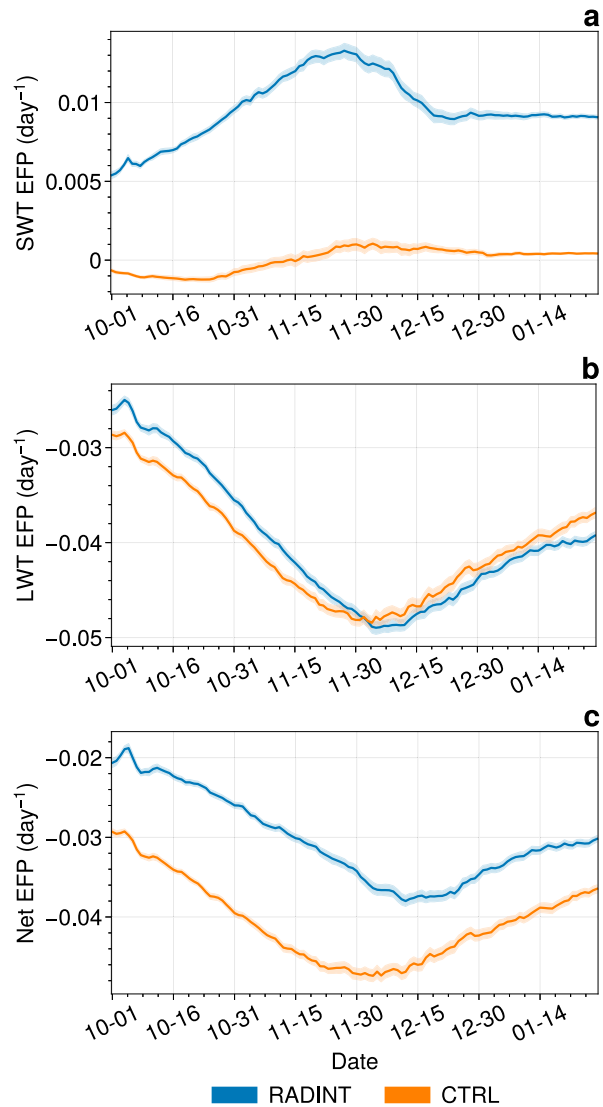
FIG. 11. EFP for SWT, LWT, and their sum (Net) all in units of per day for deviations away from the zonal mean. This is calculated at 60^\circ S and 80 hPa.
