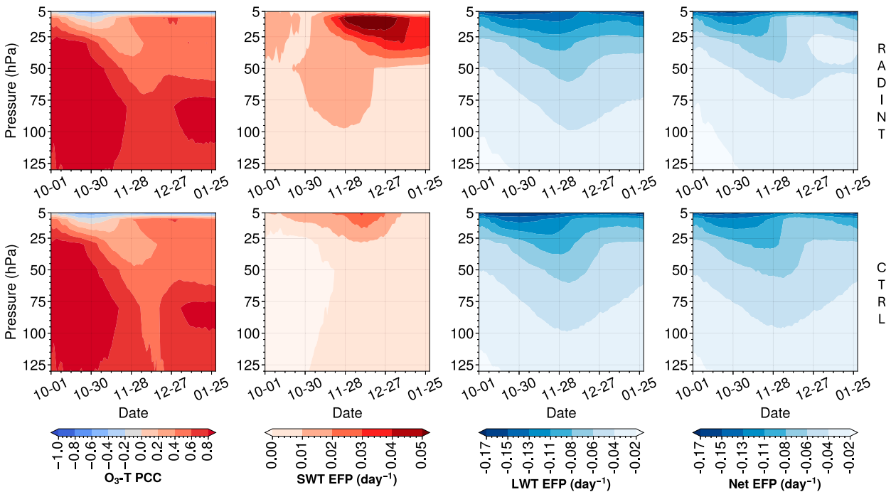
FIG. 13. (top) RADINT and (bottom) CTRL contour plots of the mean values of the (left to right) O_3 - T correlations, SWF EFP, LWT EFP, and Net EFP given as a function of height and date.
