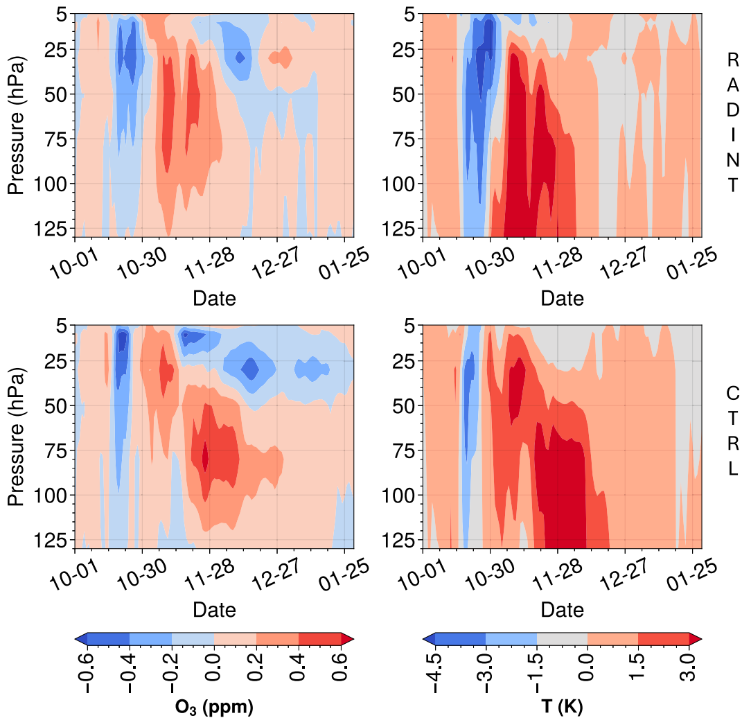
FIG. 2. Polar cap ( 60^{\circ} – 90^{\circ} S) evolution of (left) ozone (ppm) and (right) temperature (K) deviations from the ensemble mean for a single year (2018) and a single ensemble member (member 0) for (top) RADINT and (bottom) CTRL to illustrate the positive correlation between the ozone and temperature anomalies which arises from dynamical variability.
