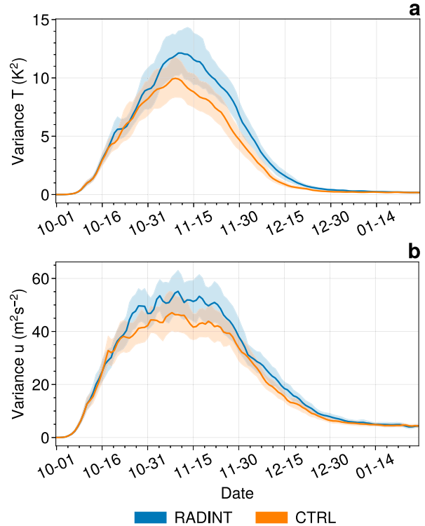
FIG. 4. The polar cap temperature ( K^2 ) and zonal-mean zonal wind ( m^2 s^{-2} ) variance with respect to the ensemble mean for RADINT (blue) and CTRL (orange). The polar cap average temperature is calculated using latitudes 60°–90°S at 80 hPa, and the zonal wind is calculated at 60°S and 50 hPa.
