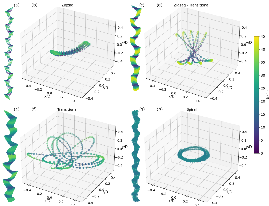
Figure 4. Case studies visualising the periodic motion sub-types. Side views of the particle motion ( a , c , e , g ) and linearly detrended centre of mass normalised by particle diameter ( b , d , f , h ) coloured by inclination angle \theta ( ^{\circ} ) for the zigzag, zigzag–transitional, transitional, and spiral cases respectively.
