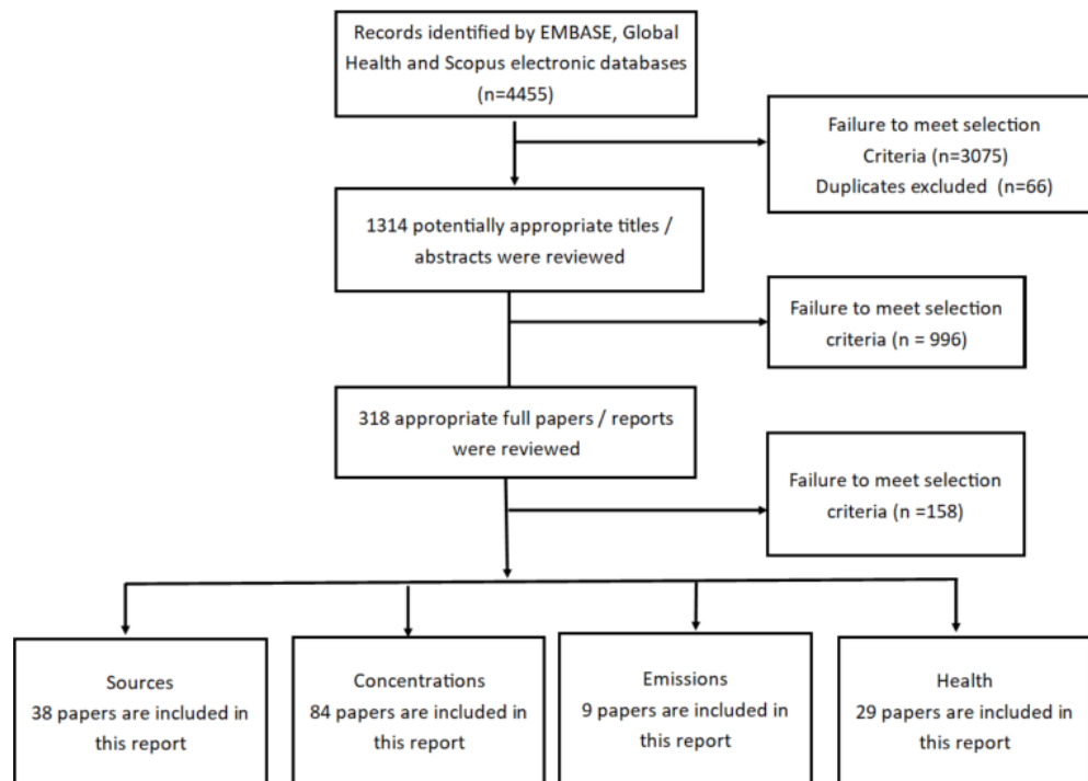
Figure 1. PRISMA diagram.
