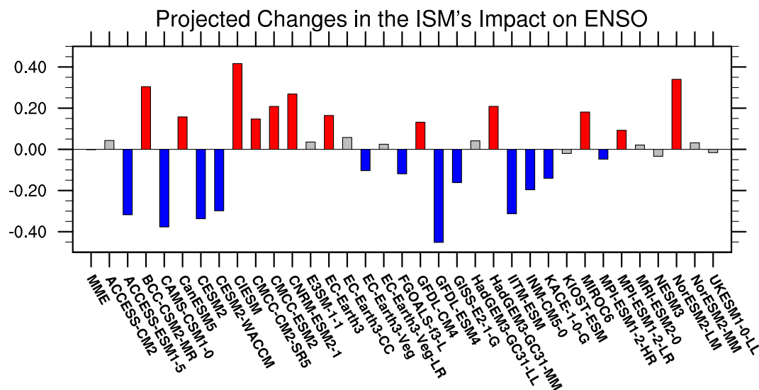
Figure 1. Projected changes in the strength of ISM impact on ENSO in the 34 CMIP6 models (units: °C), which are represented by changes in the monsoon-impact index. The red and blue bars highlight 12 models with the most significant positive and negative changes, categorized as strengthening-impact models and weakening-impact models, respectively.
