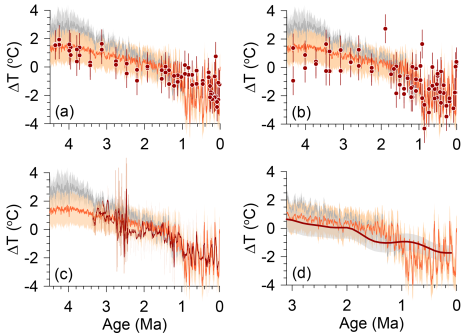
Figure 6. Our reconstructed change in mean ocean temperature ( \Delta MOT) based on HSE = 0.5 before 1.5 Ma ( 1\sigma uncertainty) and HSE = 1 after 0.9 Ma with a linear increase in HSE from 0.5 to 1 between 1.5 and 0.9 Ma (orange) compared to reconstructions of bottom water temperature anomalies ( \Delta BWT) from Mg / Ca proxies. Also shown is \Delta MOT based on HSE = 1 (gray) for the past 4.5 Ma. (a) \Delta BWT from equatorial Pacific ODP site 806 (Lear et al., 2003). Mg / Ca BWTs were mean-shifted by -1.73^\circ\text{C} to fall within same range as our \Delta MOT reconstruction for the last 800 kyr. (b) \Delta BWT from equatorial Atlantic ODP site 926 (Lear et al., 2003). Mg / Ca BWTs were mean-shifted by -1.73^\circ\text{C} so that they are referenced to the Holocene (i.e., 0^\circ\text{C} for the last 10 kyr). (c) \Delta BWT from North Atlantic DSDP site 607 for > 2.9 Ma (Dwyer and Chandler, 2009) and < 2.8 Ma (Sosdian and Rosenthal, 2009) (11-point running average in dark red) and \Delta BWT from North Atlantic IODP site U1313 for 2.4–2.75 Ma (Jakob et al., 2020). Site 607 data are mean-shifted by 2.71^\circ\text{C} so that they are referenced to the Early Holocene (i.e., 0^\circ\text{C} at 10 ka). Site U1313 data are referenced to modern BWT derived by Mg / Ca measurements on core-top sample. (d) Smoothed \Delta BWT reconstruction from Cramer et al. (2011) (dark-red line) using their Eq. (7b) with 90 % confidence interval (gray shading). BWTs were mean-shifted by 2.1^\circ\text{C} so that they have the same long-term mean as our \Delta MOT reconstruction over the last 400 kyr. The 1\sigma uncertainty on our \Delta MOT reconstructions is derived by combining in quadrature 1\sigma uncertainties on the \Delta GMSST reconstruction and on the relationship between \Delta GMSST and \Delta MOT (Fig. 2a), which closely corresponds to a range in HSE between 0.7 and 0.3 (Fig. 6b, e).
