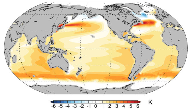
Figure 15. iTRACE ICE-only (ICE run) simulation of ocean surface temperature change (upper 10 m) for the Middle Holocene (6 ka) minus LGM.
