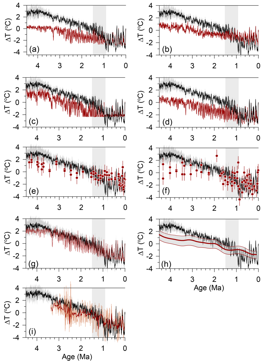
Figure 3. The reconstruction of global mean sea surface temperature change from preindustrial (Clark et al., 2024) (black with 1\sigma uncertainty in gray) compared to reconstructions of changes in bottom water temperature ( \Delta BWT, dark red). The vertical gray box represents the Middle Pleistocene Transition (0.9–1.5 Ma). (a) \Delta BWT reconstruction from Rohling et al. (2022), referenced to preindustrial (PI). (b) \Delta BWT reconstruction from Hansen et al. (2013). BWTs were mean-shifted by 1^\circ\text{C} so that they are referenced to the Holocene (i.e., 0^\circ\text{C} for the last 10 kyr). (c) \Delta BWT reconstruction from Bates et al. (2014). BWTs were mean-shifted by 1.46^\circ\text{C} so that they are referenced to the Holocene (i.e., 0^\circ\text{C} for the last 10 kyr). (d) \Delta MOT reconstruction from de Boer et al. (2014), referenced to PI. (e) Mg / Ca \Delta BWT reconstruction from ODP site 806 (Lear et al., 2003). Mg / Ca BWTs were mean-shifted by -1.73^\circ\text{C} to fall within same range as our \Delta MOT reconstruction for the last 800 kyr. (f) Mg / Ca \Delta BWT reconstruction from ODP site 926 (Lear et al., 2003). Mg / Ca BWTs were mean-shifted by -1.73^\circ\text{C} so that they are referenced to the Holocene (i.e., 0^\circ\text{C} for the last 10 kyr). (g) Deep-ocean temperature reconstruction from Evans et al. (2024), which is the Rohling et al. (2022) reconstruction (a) with pH-corrected benthic \delta^{18}\text{O} , referenced to PI. (h) The 2 Myr smoothed \Delta BWT reconstruction from Cramer et al. (2011) using their Eq. (7b) with 90 % confidence interval. BWTs were mean-shifted by 2.1^\circ\text{C} so that they have the same long-term mean as our \Delta MOT reconstruction over the last 400 kyr. (i) Mg / Ca \Delta BWT from North Atlantic DSDP site 607 for > 2.9 Ma (Dwyer and Chandler, 2009) and < 2.8 Ma (Sosdian and Rosenthal, 2009) (11-point running average in dark red) and \Delta BWT from North Atlantic IODP site U1313 for 2.4–2.75 Ma (Jakob et al., 2020). Site 607 data are mean-shifted by -1.73^\circ\text{C} so that they are referenced to the Early Holocene (i.e., 0^\circ\text{C} at 10 ka). Site U1313 data are referenced to modern BWT derived by Mg / Ca measurements on core-top samples.
