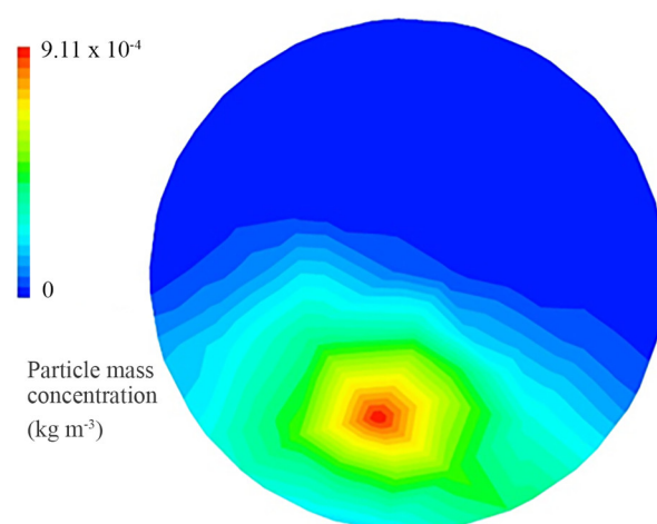
Figure 8. Distribution of particle mass concentration at the exit of the pipe.
