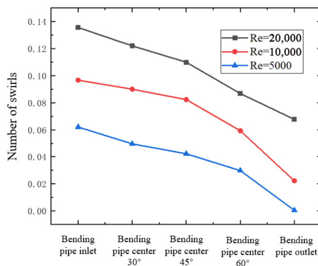
Figure 5. Variation of swirl number under different Re.
