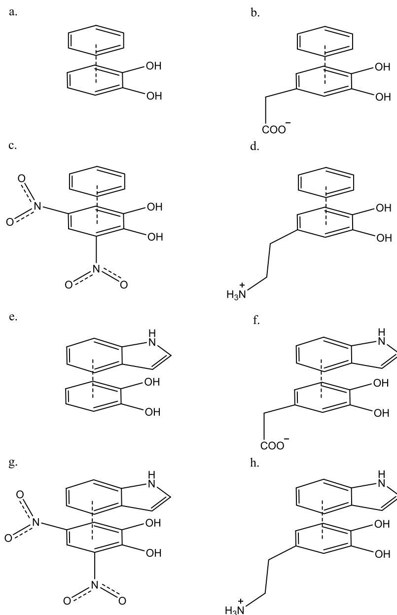
Figure 3. \pi -stacking systems used in this study: benzene stacked with (a) catechol, (b) DOPAC, (c) dinitro catechol, and (d) dopamine, and indole stacked with (e) catechol, (f) DOPAC, (g) dinitro catechol, and (h) dopamine.
