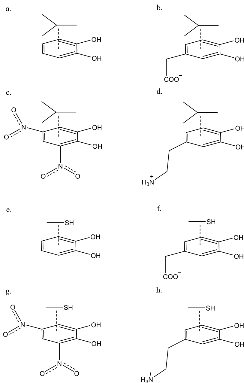
Figure 4. Other systems used in this study: isobutane complexed with (a) catechol, (b) DOPAC, (c) dinitro catechol, and (d) dopamine, and methanethiol complexed with (e) catechol, (f) DOPAC, (g) dinitro catechol, and (h) dopamine.
