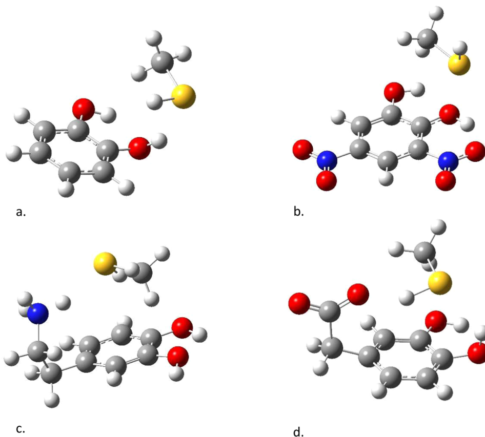
Figure 6. CCSD/cc-pVDZ optimized structures of (a) catechol-methanethiol, (b) dinitrocatechol-methanethiol, (c) dopamine-methanethiol, (d) DOPAC-methanethiol.
