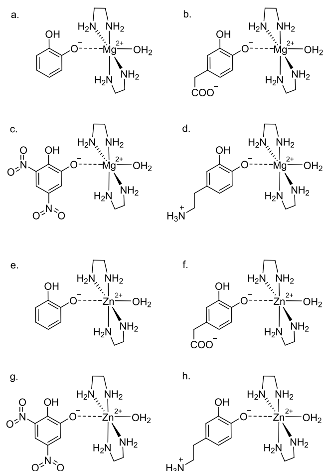
Figure 1. Metal complex model systems used in this study: \text{Mg}^{2+} in an octahedral complex with 2 ethylene diamine molecules, a water molecule, and (a) catechol, (b) DOPAC, (c) dinitro catechol and (d) dopamine, and \text{Zn}^{2+} in an octahedral complex with 2 ethylene diamine molecules, a water molecule, and (e) catechol, (f) DOPAC, (g) dinitro catechol and (h) dopamine.
