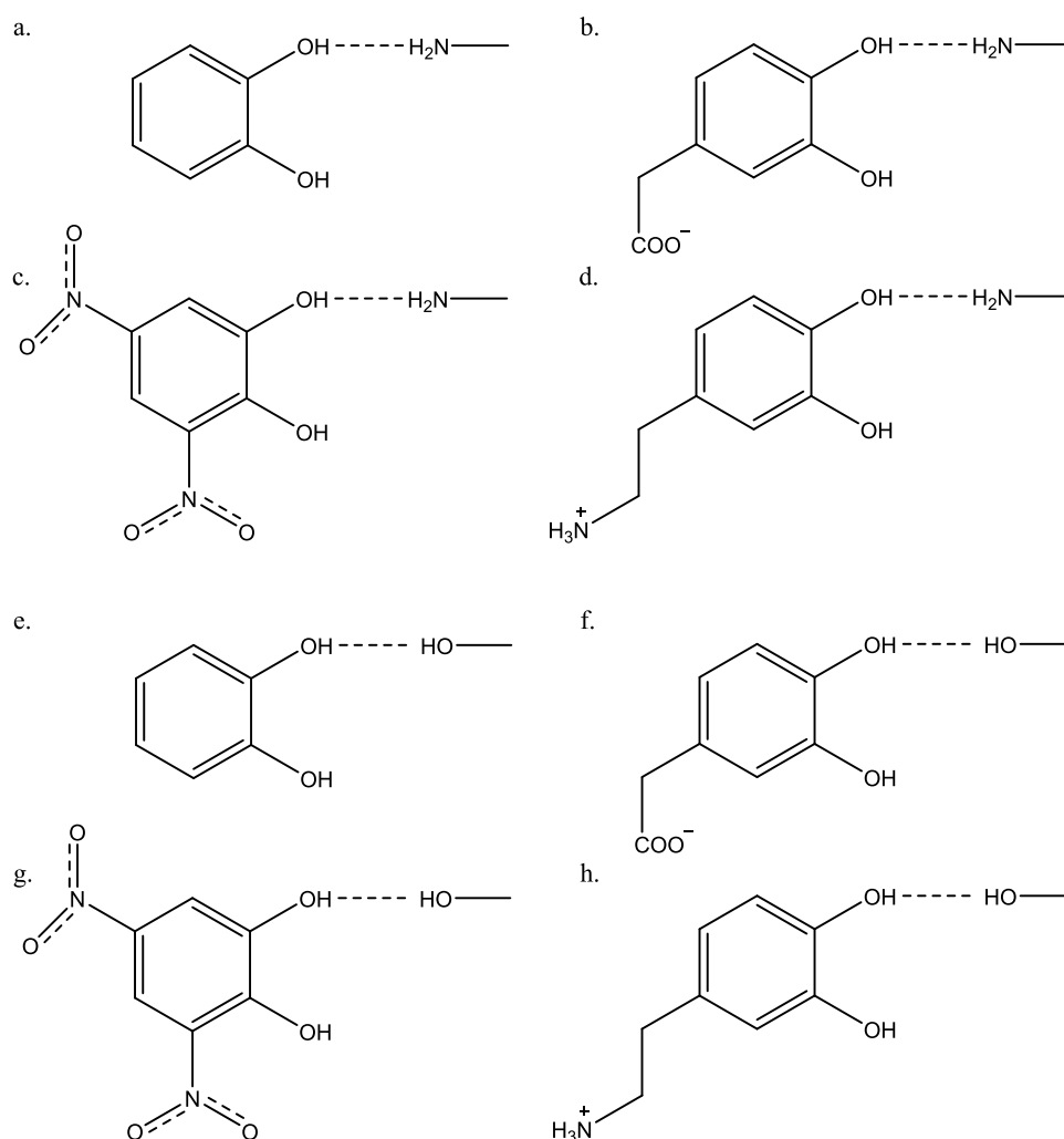
Figure 2. Hydrogen-bonded model systems used in this study: methyl amine hydrogen-bonded to (a) catechol, (b) DOPAC, (c) dinitro catechol and (d) dopamine, and methanol hydrogen-bonded to (e) catechol, (f) DOPAC, (g) dinitro catechol, and (h) dopamine.
