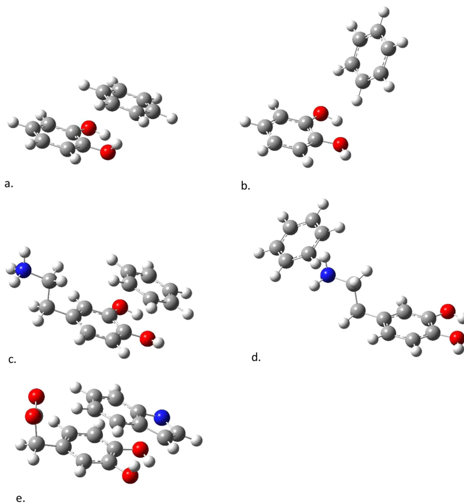
Figure 5. Optimized structures (cc-pVDZ basis set) for (a) catechol-benzene with MP2, (b) catechol-benzene with CCSD, (c) dopamine-benzene with MP2, (d) dopamine-benzene with CCSD, (e) DOPAC-indole with CCSD.
