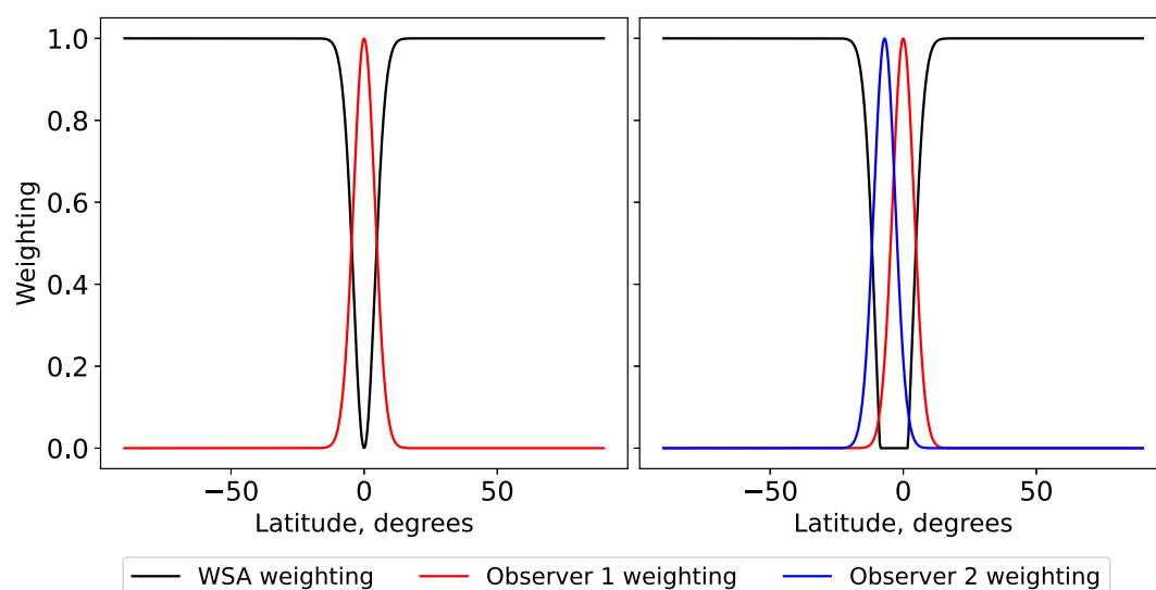
Figure 10. Example of how the WSA map and the BRaVDA posterior are weighted in latitude using a Gaussian of width 4^\circ . The left hand panel shows a single update applied by assimilating near-Earth data when the heliographic latitude was 0^\circ , with the weighting to the background WSA map in black and the weighting to the BRaVDA posterior in red. The right hand panel shows the weighting when two sources of observations are assimilated. Observer 1 (red) is located at 0^\circ latitude and Observer 2 (blue) is located at -7^\circ latitude. The WSA weighting is reduced to 0 when the total observer weighting exceeds 1 in the crossover region between the two Gaussians.
