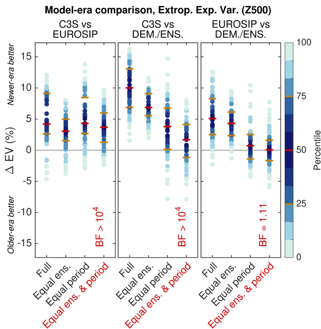
FIGURE 5 Model-era skill comparison for extratropical Northern Hemisphere Z500 anomalies for boreal winter hindcasts (DJF). The comparisons are shown for the full ensembles, as well as when controlling for equal ensemble size, equal hindcast period, and both. Each dot shows the difference between one pair of models from the different eras. The colours are shaded to show the percentile of the whole distribution and the horizontal lines show the 25th, 50th, and 75th percentiles. Also shown are the Bayes factors calculated for the median of the equal ensemble size and hindcast period distributions, which were estimated by repeated subsampling (see Section 2). [Colour figure can be viewed at wileyonlinelibrary.com ]
