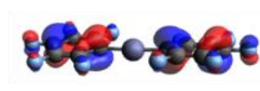
HOMO-2
