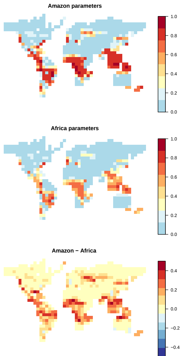
Figure 12. Maps of mean broadleaf forest fraction, over the “best” set of parameters found for the Amazon (top panel) and the Central African forest (centre panel). The difference between the two is mapped at the bottom panel.
