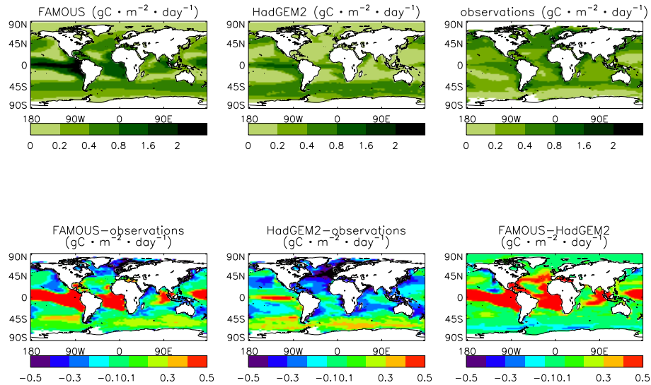
Figure 5. Net primary productivity (NPP) ( \text{gC m}^{-2} \text{ day}^{-1} ) for FAMOUS (top left), HadGEM2-ES (top middle) and observations (top right). Absolute difference plots between the models and observations are shown in the bottom left and middle left panels and the difference between the models themselves is shown in the bottom right.
