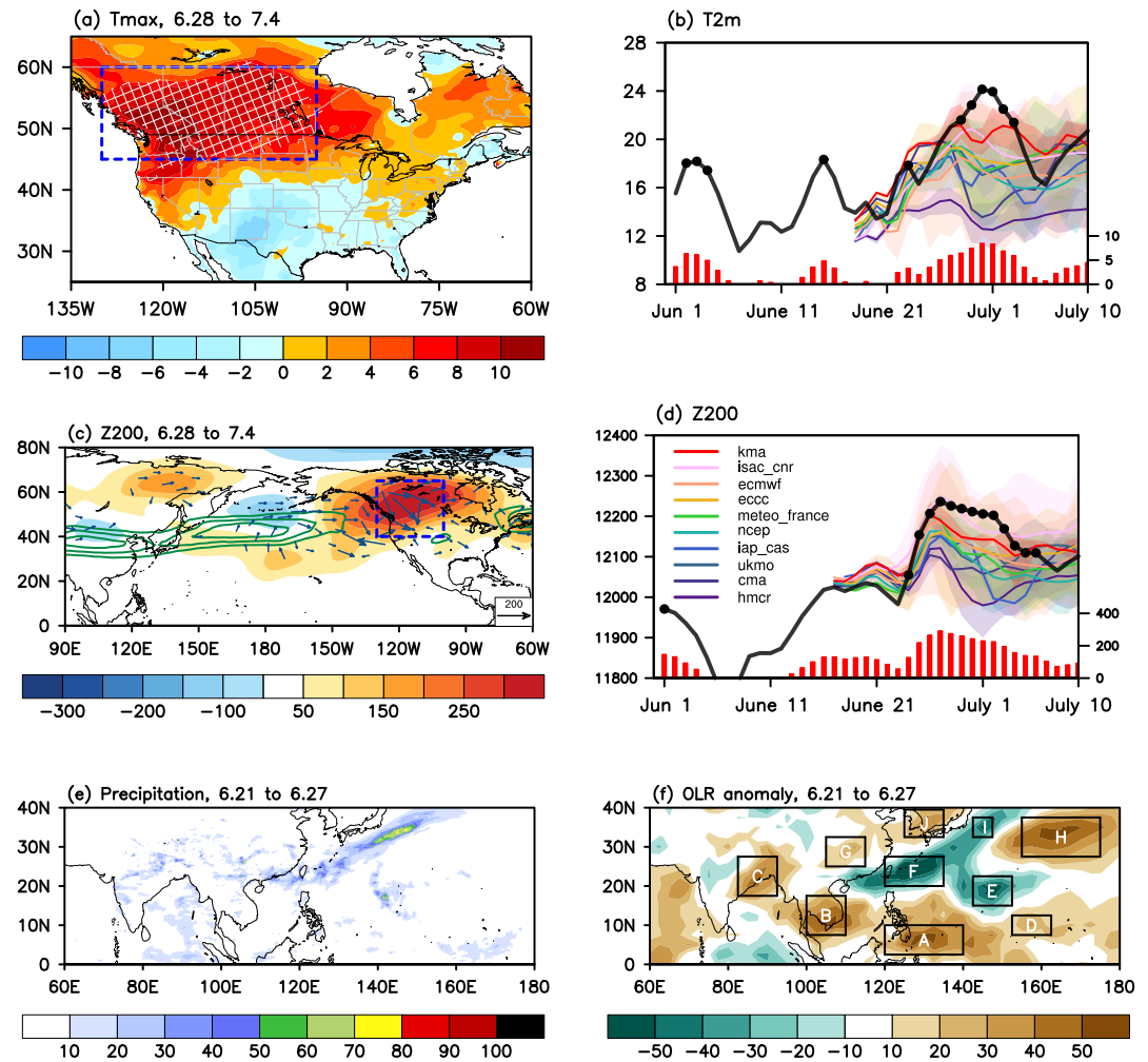
Figure 1. Characteristics of the 2021 PNW heatwave. (a) The maximum surface temperature (Tmax; °C) anomalies averaged during the peak stage of the heatwave. Hatching indicates where Tmax exceeded historical records. (b) The time evolution of daily mean surface temperature (T2m; °C) averaged over the region represented by the blue box in (a). The thick black line represents the observation, with dots indicating record-breaking values. The red bars depict the T2m anomalies and correspond to the right y-axis. Colored lines represent the multi-member mean of subseasonal-to-seasonal (S2S) predictions, where the shading represents the spread across members in each model. (c, d) Are same as (a, b), but for geopotential height at 200 hPa (Z200; gpm). In (c), green contours indicate the zonal wind speed (U200; m s -1 ), with an interval of 10 m s -1 starting from 20 m s -1 . The vectors represent the horizontal wave activity flux (Takaya & Nakamura, 2001) (m 2 s -2 ). (e) The precipitation (mm day -1 ) averaged 1 week prior to the heatwave. (f) Is same as (e), but for the outgoing longwave radiation (OLR) anomalies. The labeled sub-boxes represent the anomalous convection centers within the Asian monsoon system examined in this study.
