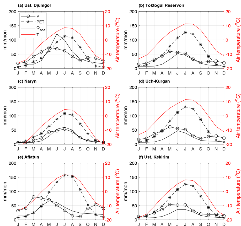
Figure 2. Climatology of monthly mean temperature ( T ), potential evaporation ( PET ), precipitation ( P ) and observed discharge ( Q_{obs} ) averaged for each sub-catchment for the calibration period 1951–1970. Temperature and PET are from the ERA5 and ERA5 back extension dataset, precipitation is from the APHRODITE dataset and observed discharge is from the Global Runoff Data Centre.
