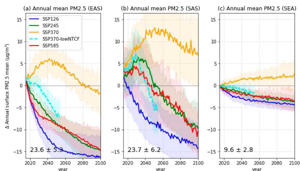
Figure 5. Future changes in the annual surface mean PM_{2.5} concentrations relative to the present-day (1995–2014) mean for various CMIP6 SSP scenarios for the three Asian regions: (a) EAS, (b) SAS, and (c) SEA. Each line represents the MME mean, and the shaded areas represent a \pm 1 standard deviation of the mean. The MME regional mean value and \pm 1 standard deviation for the present day is indicated in the bottom left corner.
