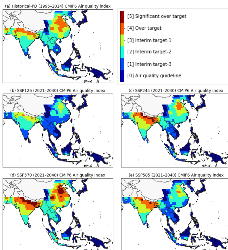
Figure 6. Spatial distribution of AQI based on WHO air-quality guidelines and interim targets for long-term exposure of PM_{2.5} for (a) the present day from CMIP6 historical simulations, and for the near future from the (b) SSP1-2.6, (c) SSP2-4.5, (d) SSP3-7.0, and (e) SSP5-8.5 scenarios. AQI value classifications are defined in Table 4.
