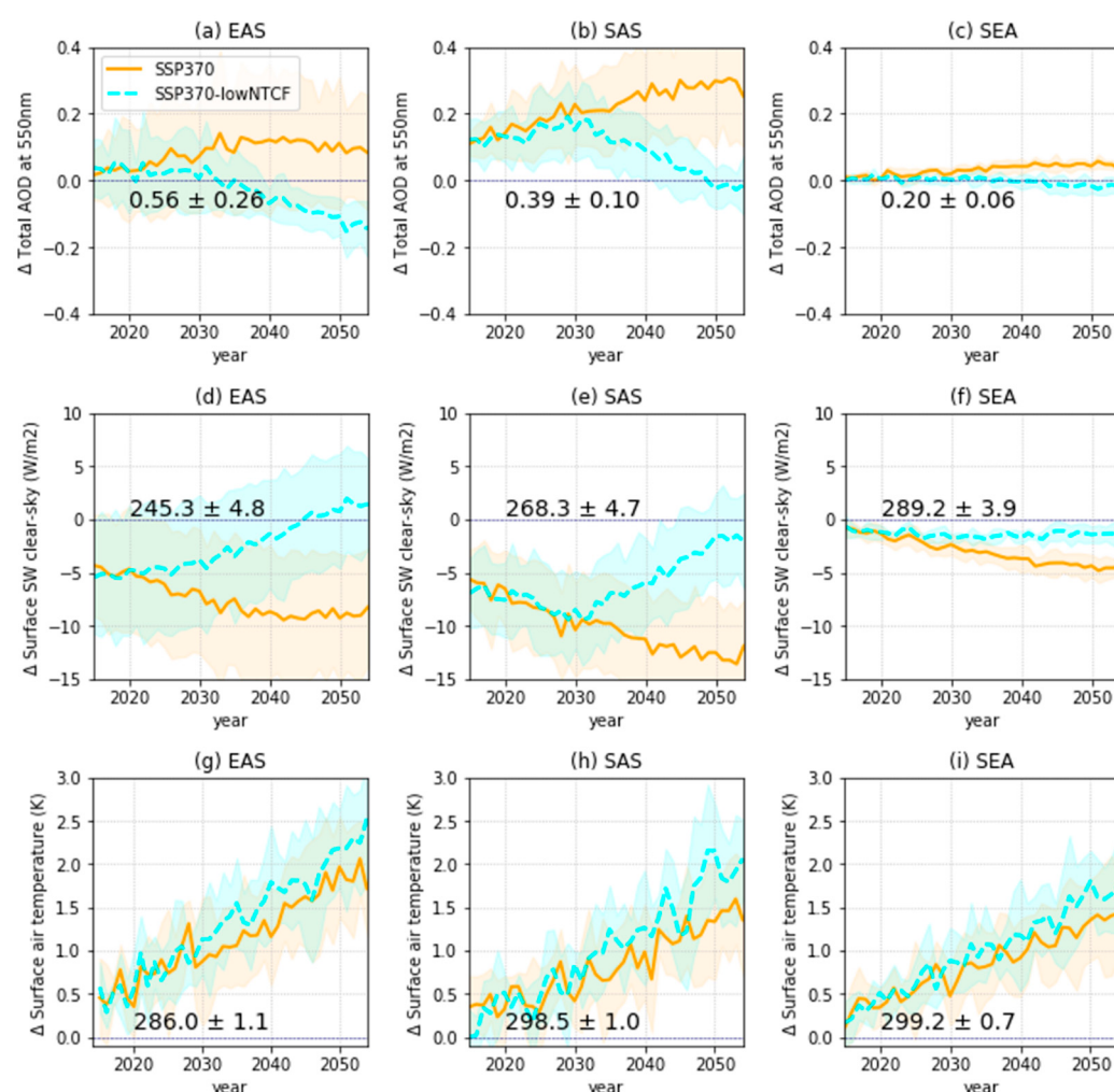
Figure 10. Future changes in annual mean total aerosol optical depths (a–c), clear-sky surface downwelling shortwave fluxes (d–f), and surface air temperatures (g–i) relative to the present-day (1995–2014) mean for the SSP3-7.0 and SSP3-7.0-lowNTCF scenarios for the three Asian regions (EAS, SAS, and SEA). Each line represents the MME mean and the shading represents the \pm 1 standard deviation of the mean. The MME regional mean value and \pm 1 standard deviation for the present day is indicated near the horizontal lines.
