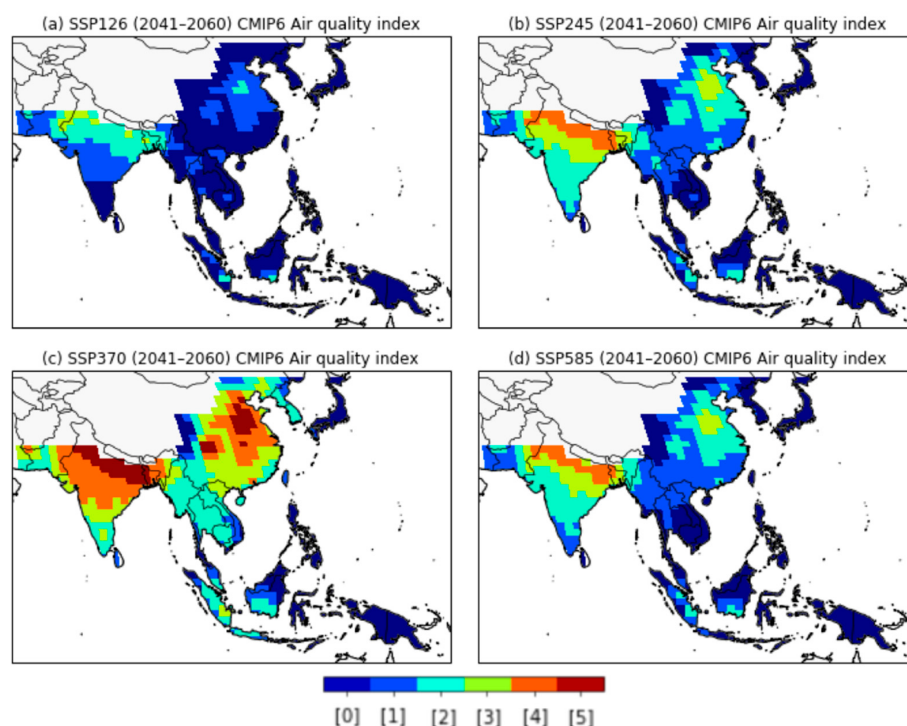
Figure 7. Spatial distribution of AQI based on WHO air-quality guidelines and interim targets for long-term exposure of PM_{2.5} for the mid-future (2041–2060) from the (a) SSP1-2.6, (b) SSP2-4.5, (c) SSP3-7.0, and (d) SSP5-8.5 scenarios. AQI value classifications are defined in Table 4.
