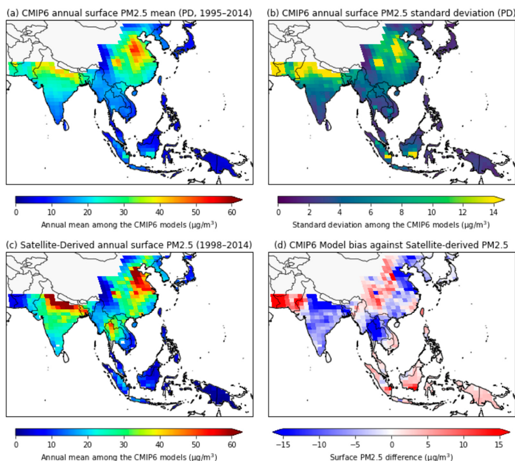
Figure 3. The spatial distribution of annual mean surface PM 2.5 concentrations from the CMIP6 historical simulations for the present-day period (1995–2014) and satellite data (1998–2014). (a) Multimodel mean, (b) standard deviation of the multimodel mean, (c) satellite-derived annual surface PM 2.5 concentrations, and (d) the difference between multimodel mean and satellite data.
