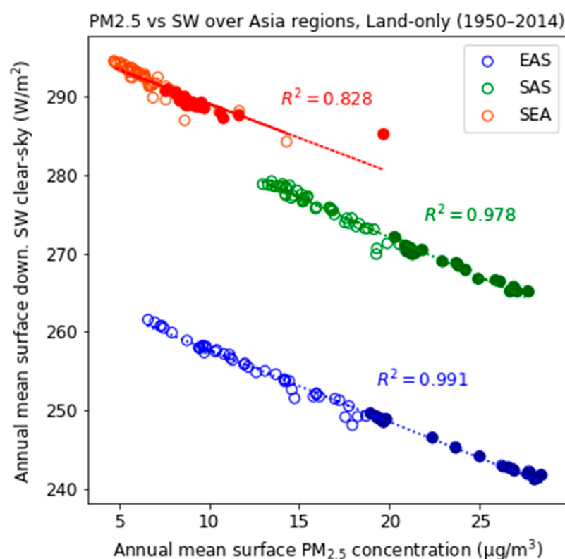
Figure 9. Scatter plot and regression line of simulated annual mean surface \text{PM}_{2.5} concentrations and clear-sky surface downwelling shortwave radiative fluxes from 1950 to 2014 for the Asian regions. The closed circles represent the ensemble mean values for the present-day period (1995–2014).
