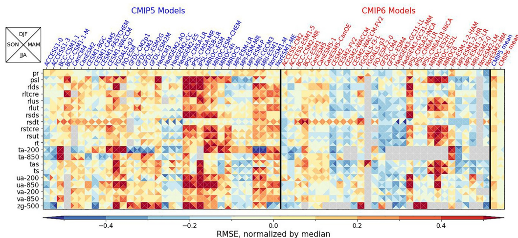
Figure 5. Overview scores for CMIP5 (left-hand side) and CMIP6 (right-hand side) models generated by the PCMDI Metrics Package, for the seasonal climatology of multiple atmospheric variables evaluated against observational data sets over the period of 1981–2005. Included here are a subset of models from institutions that participated in both CMIP5 and CMIP6 historical experiments, in order to trace changes from one multi-model ensemble to the next. CMIP5 models are labeled in blue and CMIP6 in red. Root Mean Squared Error (RMSE) values are calculated against reference data sets for each season and normalized by the median value of each row. Thus the normalized RMSE value indicates performance relative to other models within a given row, with negative values indicating a better agreement with observations. Detailed analysis information can be found in J. Lee et al. (2024) (J. Lee, 2025).
