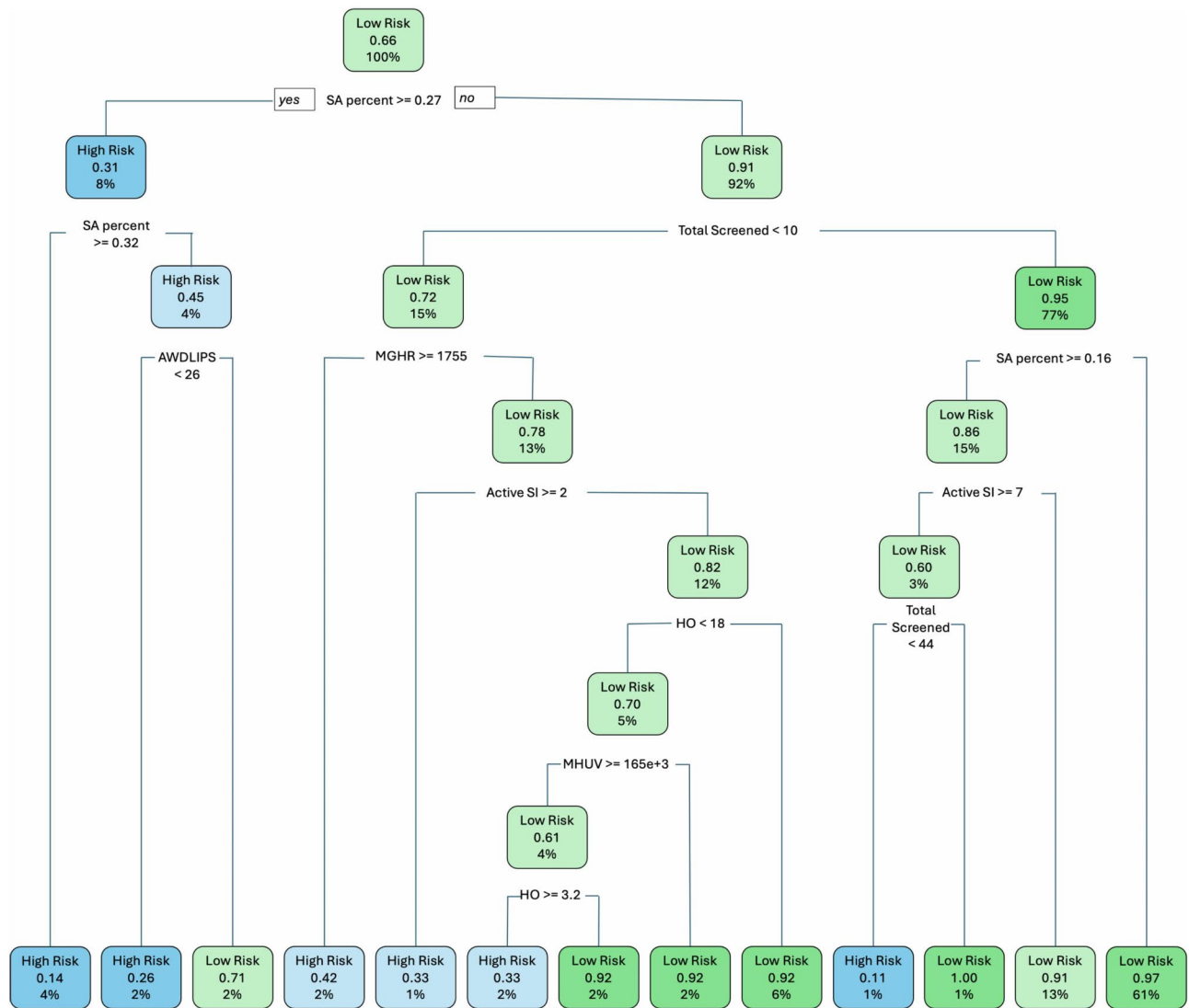
Fig. 2 Classification Tree for Predicting High and Low Suicidal Ideation Risk Census Tracts. Note. SApercent=percentage of positive suicide attempt screens; TotalScreened=total number of suicide attempt or ideation screens in census tract; AWDLIP5= 5 year average percentage of adults aged 20–64 living with a disability and below poverty level; MHGR=median household gross rent; HO=percentage of all housing units (i.e., occupied and unoccupied) that are occupied by homeowners; MHUV=median housing unit value
