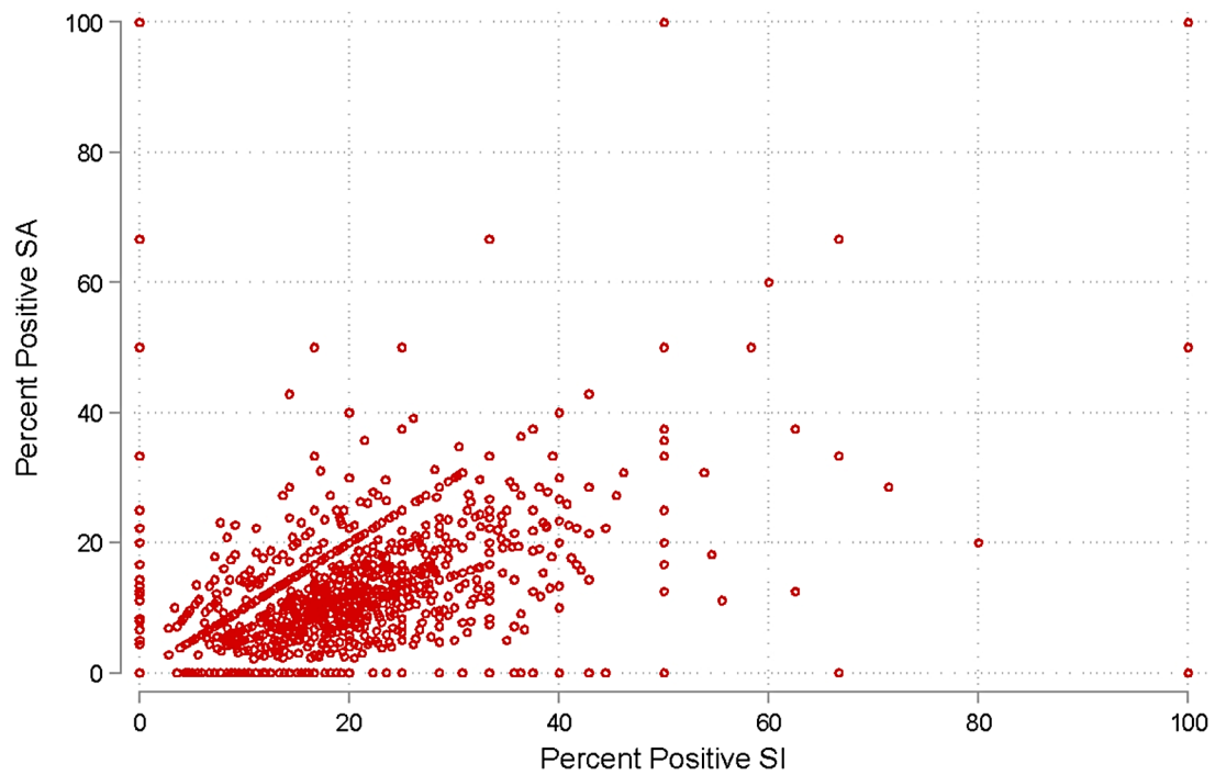
Fig. 1 Evidence of Multicollinearity and Extreme Outliers. Note. SA = suicide attempts; SI = suicidal ideation
