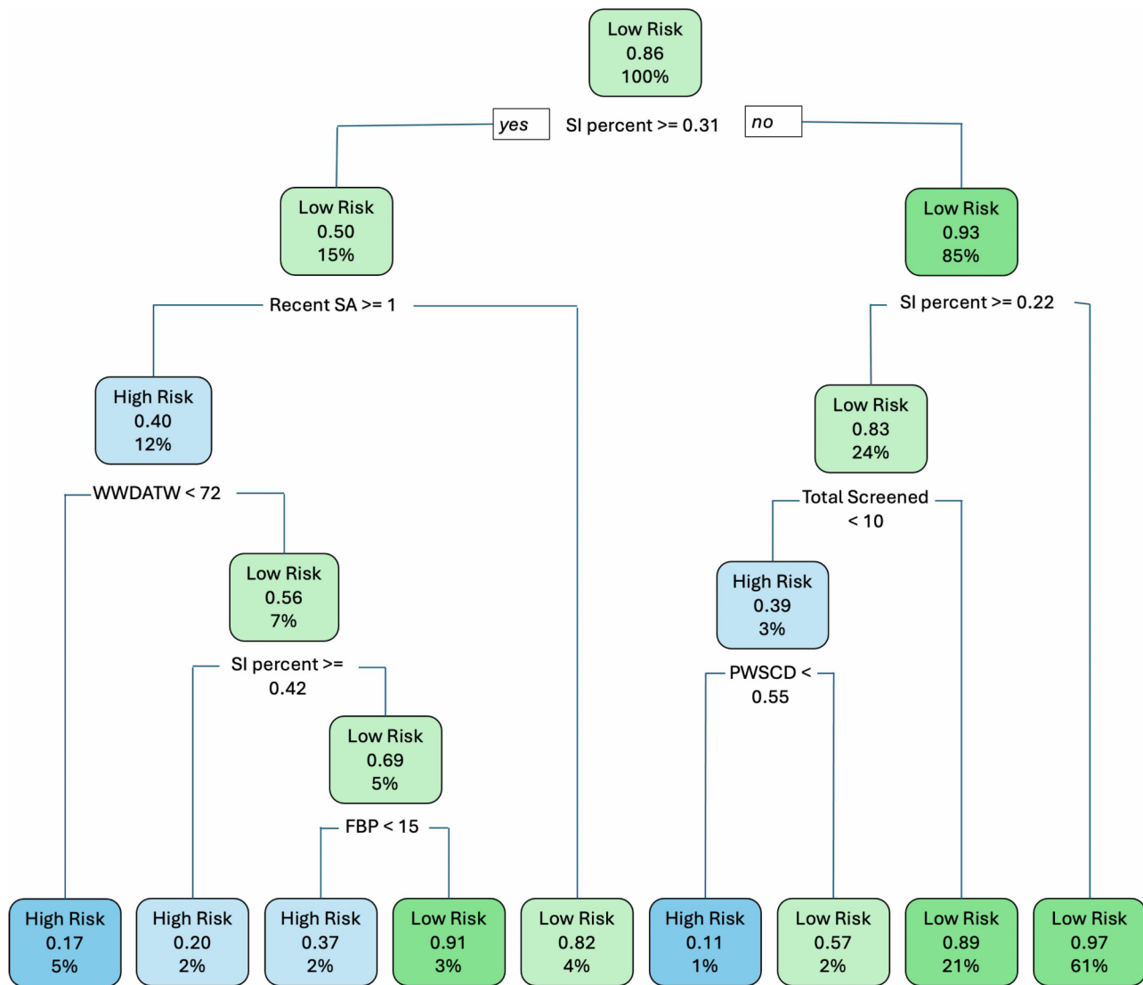
Fig. 3 Classification Tree for Predicting High and Low Suicide Attempt Risk Census Tracts. Note. SIpercent=percentage of positive suicidal ideation screens; RecentSA=number of recent suicide attempts reported; WWDATW=percentage of workers aged 16 years and over who get to work by driving alone in a car, truck, or van; PWSCD=percentage of the population with a self-care difficulty; FBP=percentage of the population who are a foreign born (persons not born in the United States, including all foreign born persons regardless of whether they are naturalized U.S. citizens)
