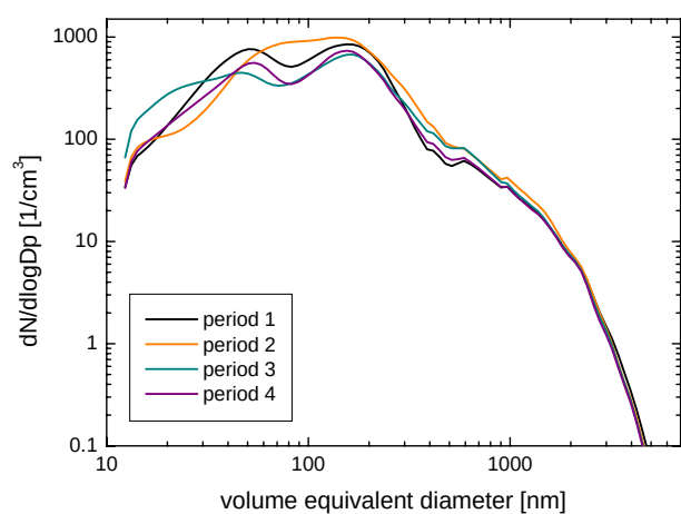
Fig. 11. Aerosol particle number size distributions averaged across each of the air mass periods during the RHaMBLe intensive project.
