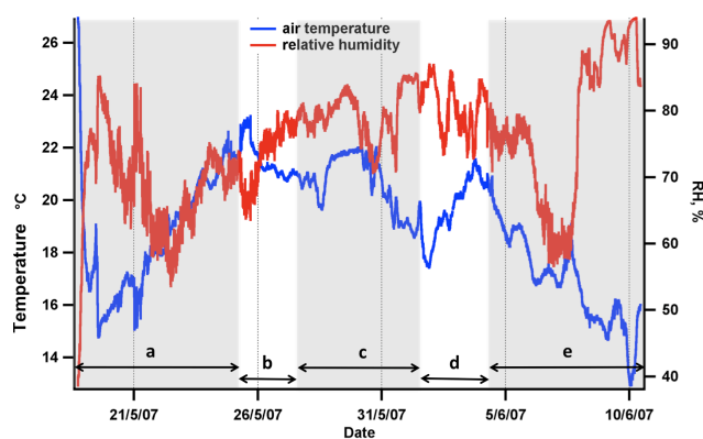
Fig. 4. Temperature and RH throughout D319. The time series are shaded according to several discrete period (a) transect from Lisbon to CV with port call in Mindelo, (b) eastward transit towards African coast, (c) detailed survey of biologically productive “Mauritanian upwelling” waters, (d) northerly “zig-zag” in and out of productive waters, (e) transit home to Falmouth from the Canaries.
