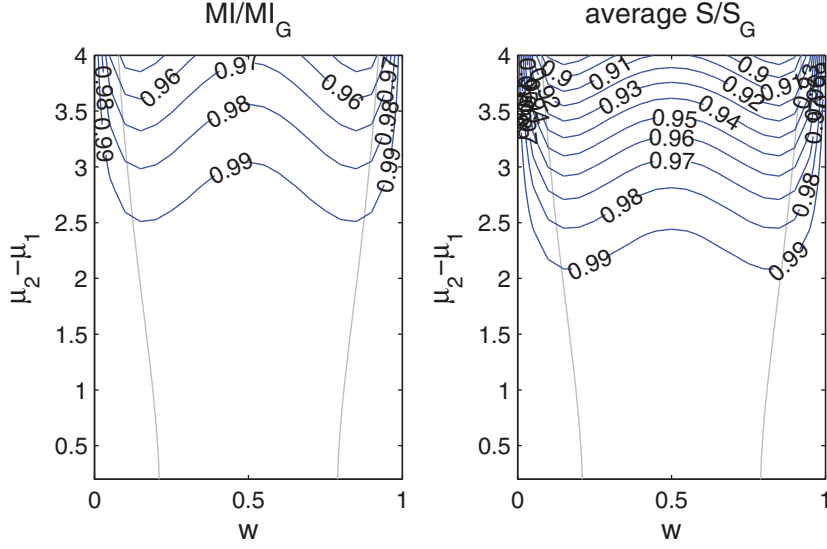
Fig. 4. Contour plots of MI (left) and \int p(y)S dy (right) all normalised by their Gaussian approximations. These are given as a function of \mu_2 - \mu_1 ( y -axis) and w ( x -axis). \sigma^2 = 1 , k = 2 . The grey lines mark the peak in the skewness (both positive and negative) of the prior.
