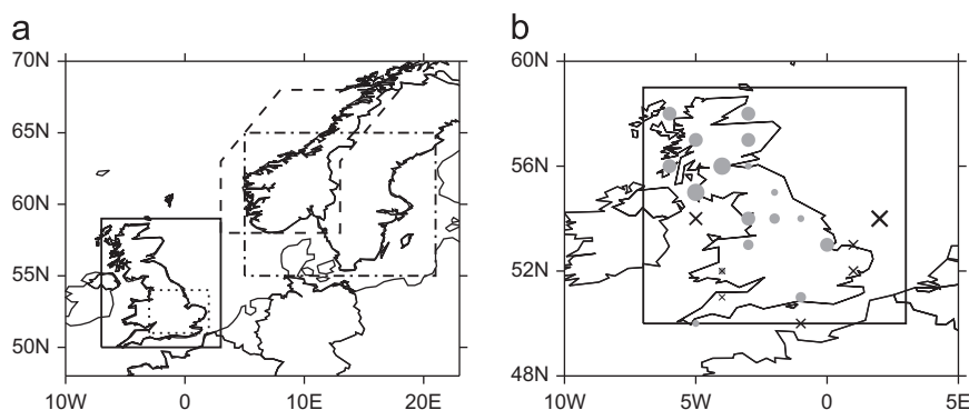
Fig. 2. (a) The power regions used in the study; UK-S (solid); UK-D (dotted); Nor-S (dashed); Sca-D (dot-dashed) and (b) the location of wind power generation capacity within UK-S, on a 1^\circ grid, onshore (grey circles) and offshore (black crosses). Symbol size is determined by the 2010 capacity, in ranges < 0.1 GW, 0.1 – 0.2 GW, 0.2 – 0.5 GW and 0.5 – 1.0 GW.
