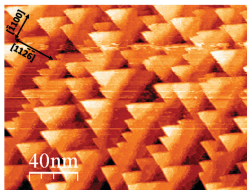
Fig. 5 The Re(11 \bar{2} 1) surface with a medium oxygen coverage (20 L O _2 adsorbed at 300 K vacuum annealed at 1000 K for 2 minutes, imaged at 1 V and 1 nA). The surface has now departed from planar and shows an ordered array of microfacets which is a precursor to the fully faceted surfaces. The measured oxygen coverage is approximately 1 ML, 1.8 \times 10^{15} atoms cm ^{-2} .
