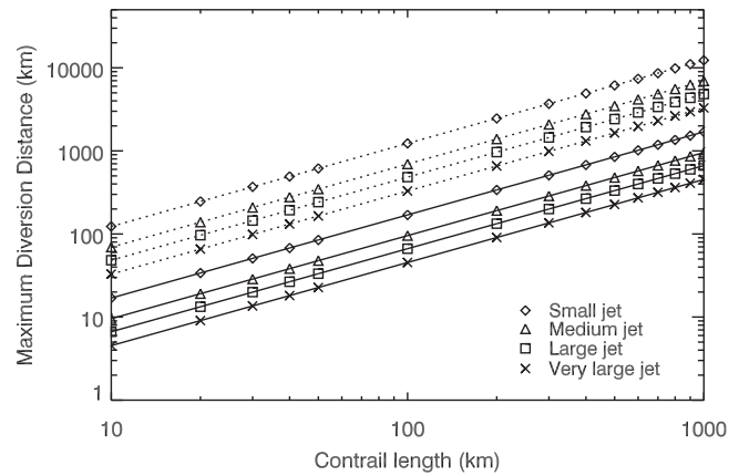
Figure 2. dx_{max} as a function of contrail length for AGWP (dotted line) and AGTP (solid line) metrics for a time horizon of 100 years. The calculations use a contrail width of 1 km.
