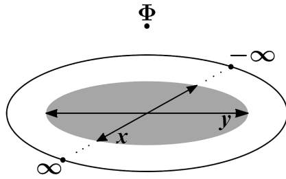
Figure 1: The transreal numbers, being the extended x -axis and the point at nullity, \Phi , as a subset of the transcomplex numbers.
