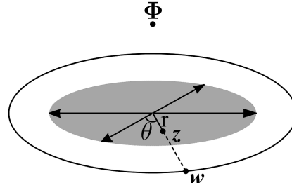
Figure 2: Entire transcomplex plane described by polar co-ordinates: z = (r, \theta) and w = (\infty, \theta) and \Phi = (\Phi, \Phi) with r, \theta finite.
