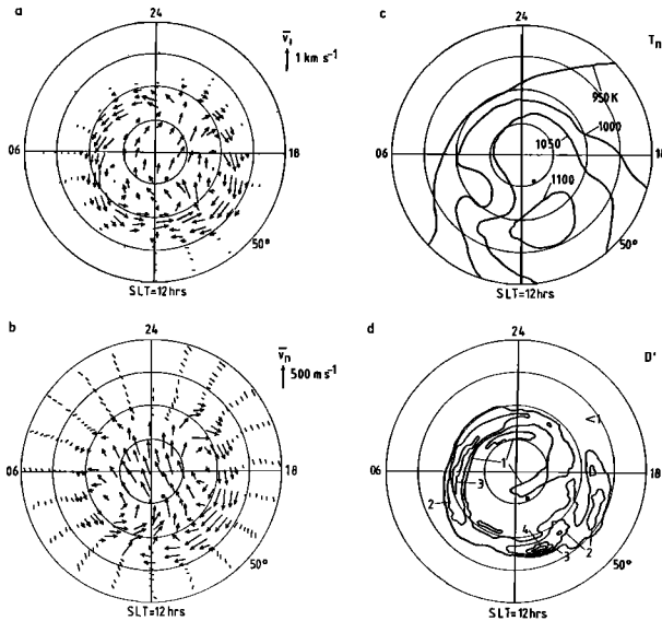
Fig. 1. Model values for the northern hemisphere at 300 km for 18 UT and December solstice with F_{10.7}=165 , K_p=3 and B_y < 0 and shown as a function of Solar Local Time (SLT) and geographic latitude over the range 50-90^\circ . The position of the magnetic pole is denoted by a dot. (a) Ion velocity vectors, \bar{v}_i ; (b) equilibrium neutral winds, \bar{v}_n ; (c) neutral temperature, T_n ; and (d) the ratio D' .
