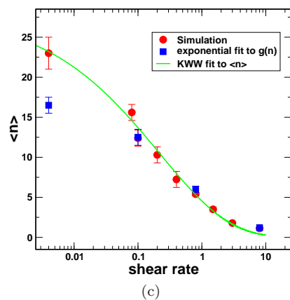
FIG. 5. For strong dipolar interaction strength \lambda \approx 6.17 : (a) the cluster size distribution g(n) as a function of chain size n for various shear rates (b) The connectivity C(n_c) as a function of coordination number n_c for various shear rates (c) average chain size \langle n \rangle as a function of shear rate. Explanation given in Sec. IV C.
