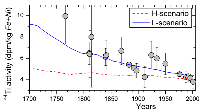
Fig. 16. Time profile of the ^{44}\text{Ti} activity in units of disintegrations per minute per kg of iron and nickel in the meteorite. The grey dots with error bars are the measurements (Taricco et al. 2006). The coloured curves depict the computed activity for the two scenarios (see text).
