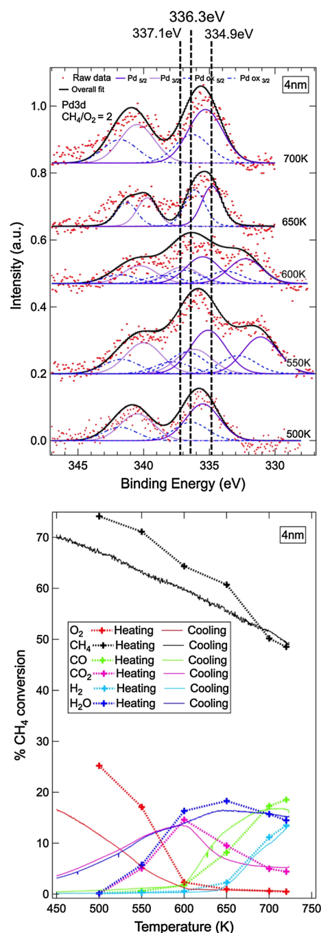
Fig. 1 Catalyst A (Pd/Al 2 O 3 nanoparticles of average size 4 nm). NAP-XPS spectra in the Pd 3d region ( top ) and CH 4 conversion, calculated from mass spectroscopy data ( bottom ), recorded in the temperature range from 450 to 720 K under 240 mTorr O 2 :CH 4 pressure (1:2). "Heating": mass spectrometry at constant temperature during NAP-XPS measurements; "Cooling": recorded during continuous cooling from 720 to 450 K. Binding energies are corrected to corresponding Al 2p spectra at 74.5 eV.
