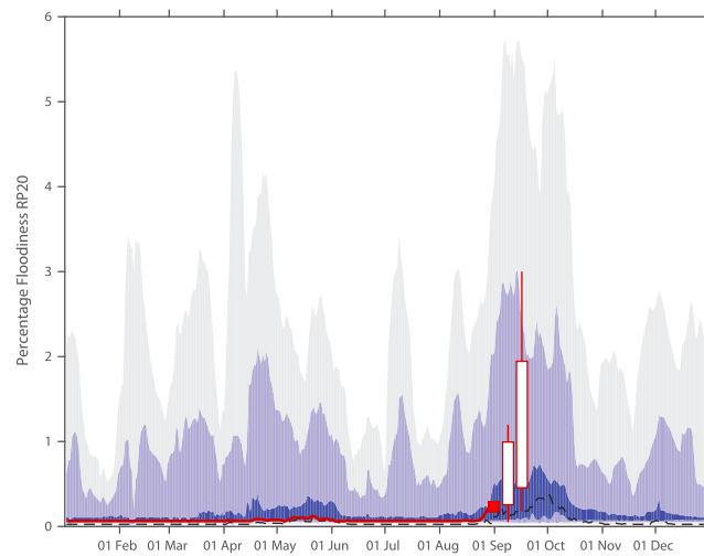
Figure 4. A climatology of 20 year return period percentage floodiness (1980–2010) for the East Africa Giorgi region. Light purple = 5th to 95th percentile, Dark purple = 33rd to 67th percentiles, Light grey = full range. A mock-up weekly floodiness forecast is shown in red.
