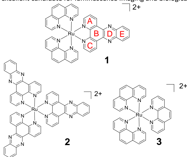
Fig. 1 The chemical structure of the 1 , 2 and 3 showing ring lettering codes used to describe the dppz ligand.
