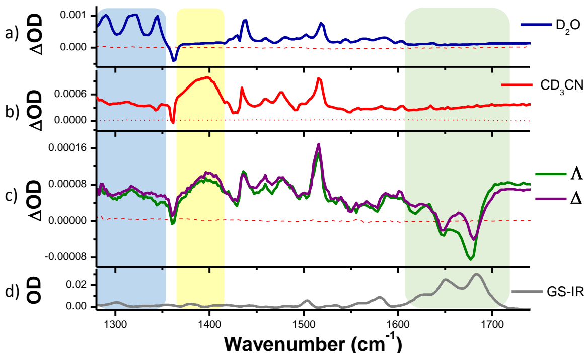
Fig. 8 TRIR spectra recorded 35 ps after 400 nm excitation of a) 1 ·2Cl (500 \mu M) in D 2 O, b) 1 ·2PF 6 (500 \mu M) in CD 3 CN and c) \Lambda - and \Delta -[ 1 ]2Cl + (400 \mu M) and a duplex DNA oligonucleotide d(TCGGCGCCGA) 2 (500 \mu M duplex) and d) FTIR spectrum oligonucleotide d(TCGGCGCCGA) 2 (500 \mu M duplex) in deuterated potassium phosphate buffer (50 mM) pH 7. The blue and yellow coloured regions highlight the characteristic transient bands for the excited state of 1 , while the green coloured region highlights the bands associated with the base DNA base pairs.
