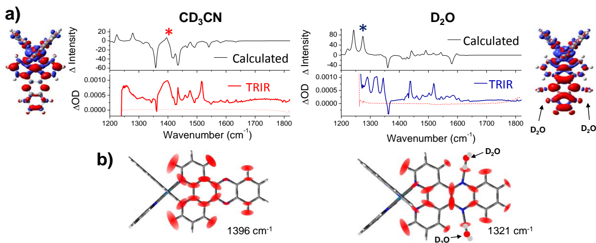
Fig. 7 a) Simulated difference spectra compared with the experimental TRIR spectra of 1 in acetonitrile (left column); and 1 -2(D 2 O) in water (right column). In the experimental spectra, wavenumbers below 1250 cm -1 were inaccessible due to strong absorbance of both solvents in this region. Structural inserts show electron density difference map (iso level 0.0008) between the lowest energy triplet state of 1 minus the electron density of the equivalent singlet ground-state at the same geometry in acetonitrile (left hand side) and for 1 -2(D 2 O) in water (right hand side). (The red and blue volumes indicate the regions where the electron density is respectively higher and lower in the triplet state compared to the ground state); b) Graphical illustration of the in-plane vibrational modes of the marker bands of the “bright” and “dark” states of 1 at 1396 cm -1 in CD 3 CN and 1321 cm -1 in D 2 O (marked with asterisks in the spectra). Red ellipsoids indicate the regions of largest atomic displacement. Animations of these vibrations can be found online in the ESI † (Animation 1-CD 3 CN and Animation 2-D 2 O).
