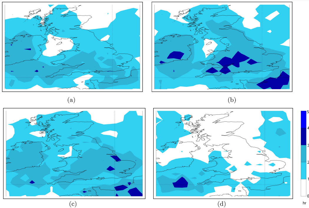
Figure 8. The average convective adjustment timescale for JJA 2012-2014 at a) T+6-T+9 (0900–1200 UTC), b) T+9-T+12 (1200–1500 UTC), c) T+12–15 (1500–1800 UTC) and d) T+18-T+21 (2100–0000 UTC) where the colour scale refers to all plots.
