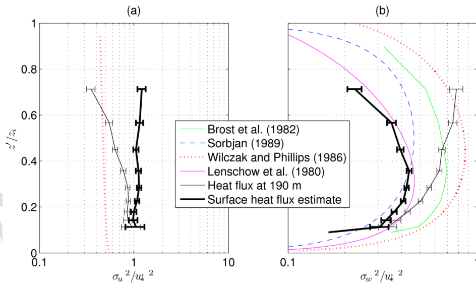
Fig. 8 Normalized standard deviations of u (a) and w (b) (kinematic heat flux at BT Tower ( \overline{w'T}_{190} ) and estimated for the surface ( \overline{w'T}_0 ) have been used to scale data) as a function of binned z'/z_i . Confidence intervals (95%) of the means are shown (data sub-sampled for daytime, cases of stronger convection ( \zeta < -0.5 ), \bar{U} > 1 \text{ m s}^{-1} and |\overline{w'T}| > 0.01 \text{ K m s}^{-1} )
